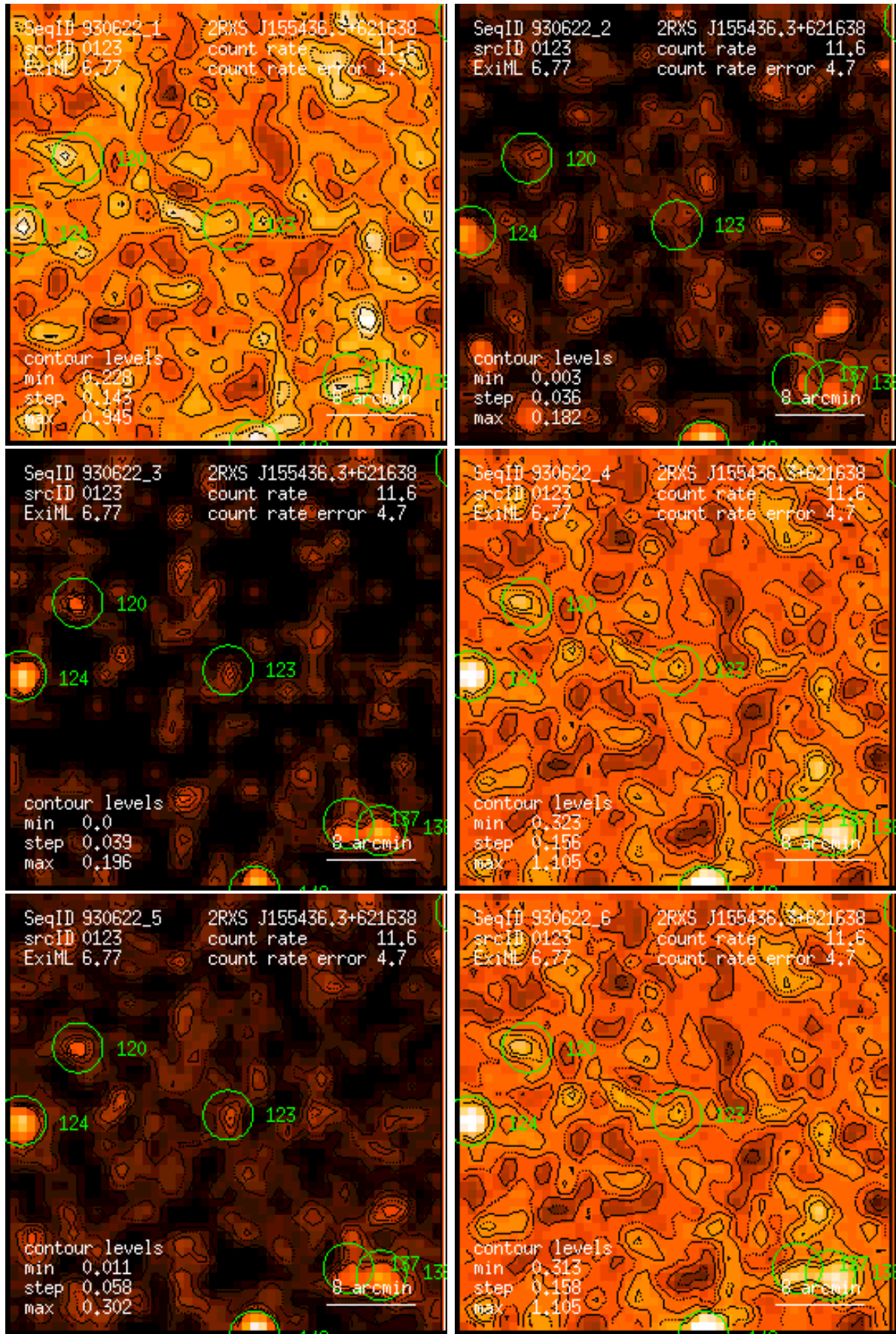
Figure 123: RASS 930622: detection 0123: band rate images, Gaussian filter: (1) PSPC channels 11 – 41, (2) 52 – 90, (3) 91 – 201, (4) 11 – 235, (5) 52 – 201, (6) 11 – 201. Broad band rates in counts/ks. Band rate contour levels in counts/ks/arcmin 2 .
