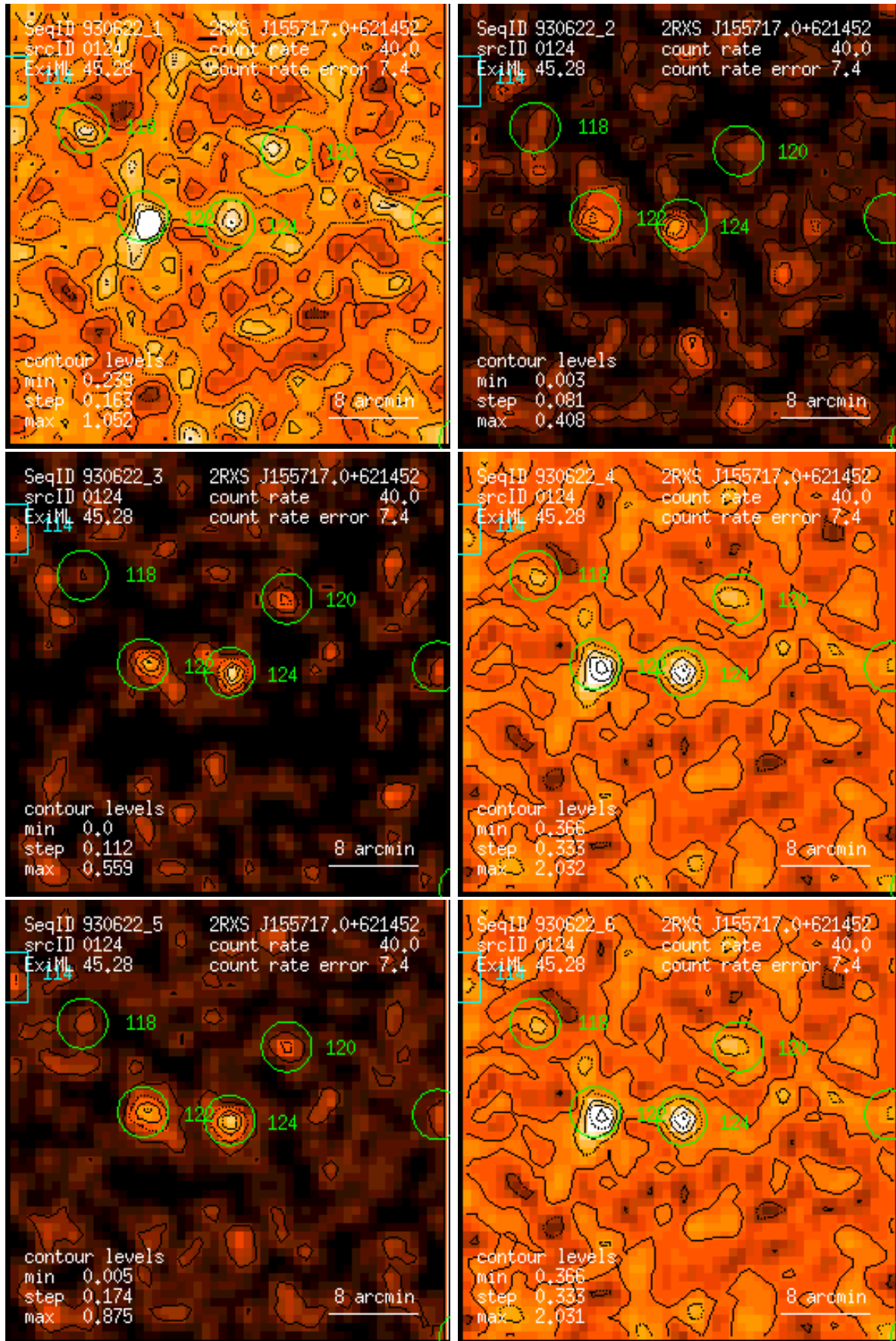
Figure 124: RASS 930622: detection 0124: band rate images, Gaussian filter: (1) PSPC channels 11 – 41, (2) 52 – 90, (3) 91 – 201, (4) 11 – 235, (5) 52 – 201, (6) 11 – 201. Broad band rates in counts/ks. Band rate contour levels in counts/ks/arcmin 2 .
