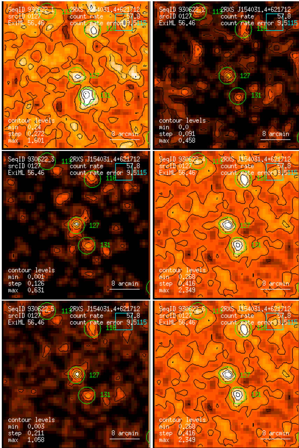
Figure 127: RASS 930622: detection 0127: band rate images, Gaussian filter: (1) PSPC channels 11 – 41, (2) 52 – 90, (3) 91 – 201, (4) 11 – 235, (5) 52 – 201, (6) 11 – 201. Broad band rates in counts/ks. Band rate contour levels in counts/ks/arcmin 2 .
