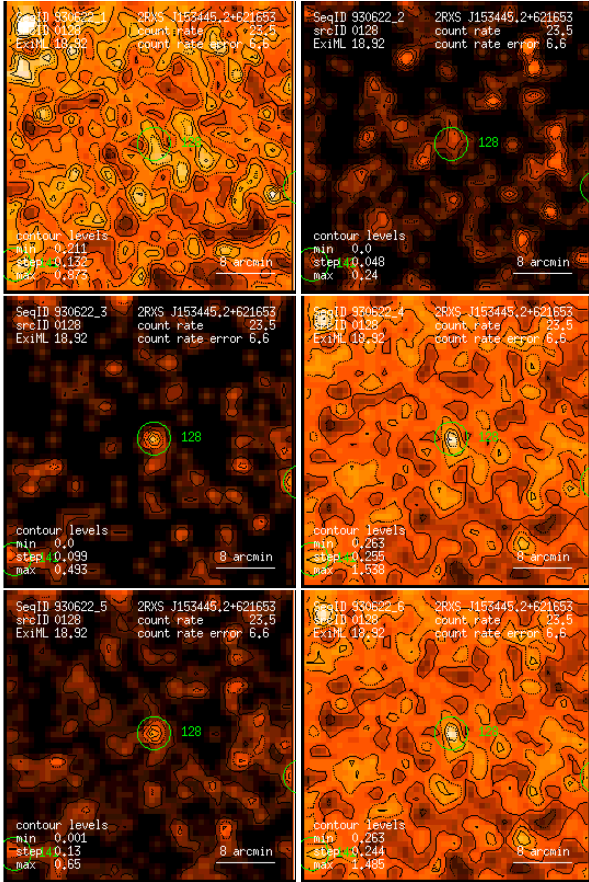
Figure 128: RASS 930622: detection 0128: band rate images, Gaussian filter: (1) PSPPC channels 11 – 41, (2) 52 – 90, (3) 91 – 201, (4) 11 – 235, (5) 52 – 201, (6) 11 – 201. Broad band rates in counts/ks. Band rate contour levels in counts/ks/arcmin 2 .
