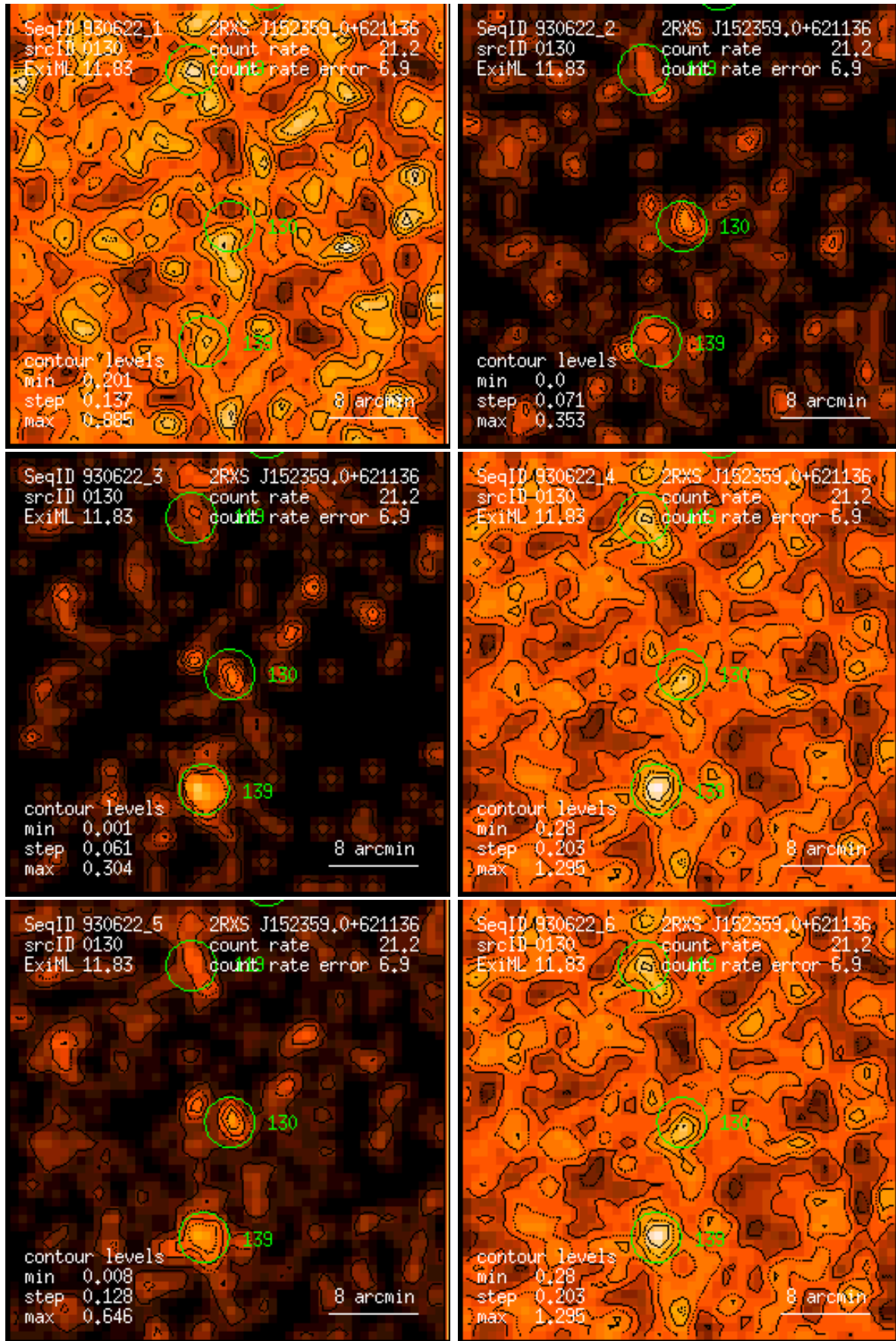
Figure 130: RASS 930622: detection 0130: band rate images, Gaussian filter: (1) PSPC channels 11 – 41, (2) 52 – 90, (3) 91 – 201, (4) 11 – 235, (5) 52 – 201, (6) 11 – 201. Broad band rates in counts/ks. Band rate contour levels in counts/ks/arcmin 2 .
