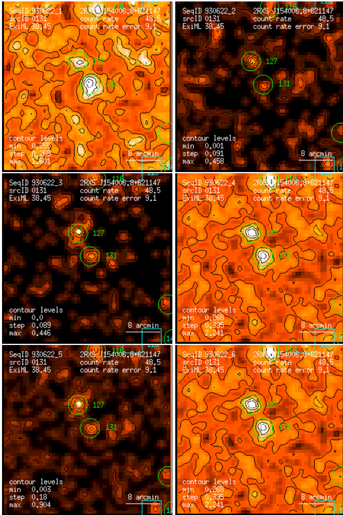
Figure 131: RASS 930622: detection 0131: band rate images, Gaussian filter: (1) PSPC channels 11 – 41, (2) 52 – 90, (3) 91 – 201, (4) 11 – 235, (5) 52 – 201, (6) 11 – 201. Broad band rates in counts/ks. Band rate contour levels in counts/ks/arcmin 2 .
