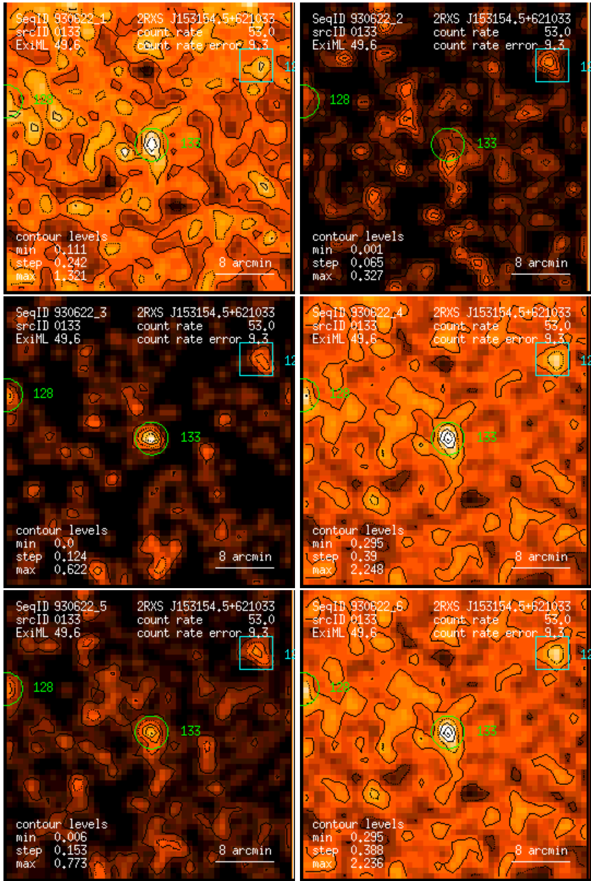
Figure 133: RASS 930622: detection 0133: band rate images, Gaussian filter: (1) PSPC channels 11 – 41, (2) 52 – 90, (3) 91 – 201, (4) 11 – 235, (5) 52 – 201, (6) 11 – 201. Broad band rates in counts/ks. Band rate contour levels in counts/ks/arcmin 2 .
