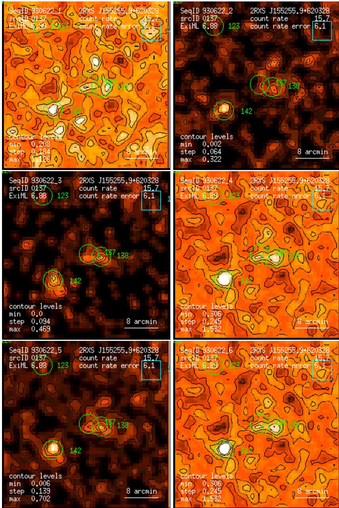
Figure 137: RASS 930622: detection 0137: band rate images, Gaussian filter: (1) PSPC channels 11 – 41, (2) 52 – 90, (3) 91 – 201, (4) 11 – 235, (5) 52 – 201, (6) 11 – 201. Broad band rates in counts/ks. Band rate contour levels in counts/ks/arcmin 2 .
