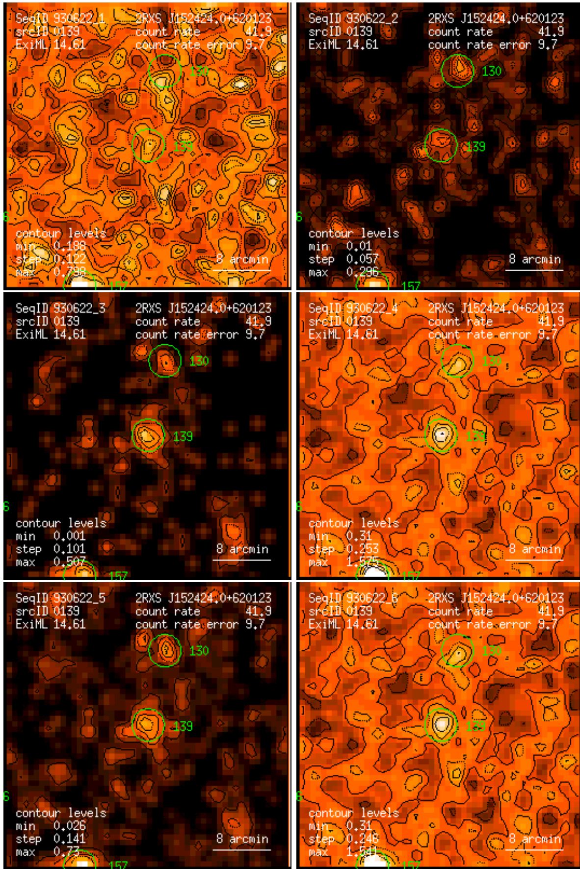
Figure 139: RASS 930622: detection 0139: band rate images, Gaussian filter: (1) PSPC channels 11 – 41, (2) 52 – 90, (3) 91 – 201, (4) 11 – 235, (5) 52 – 201, (6) 11 – 201. Broad band rates in counts/ks. Band rate contour levels in counts/ks/arcmin 2 .
