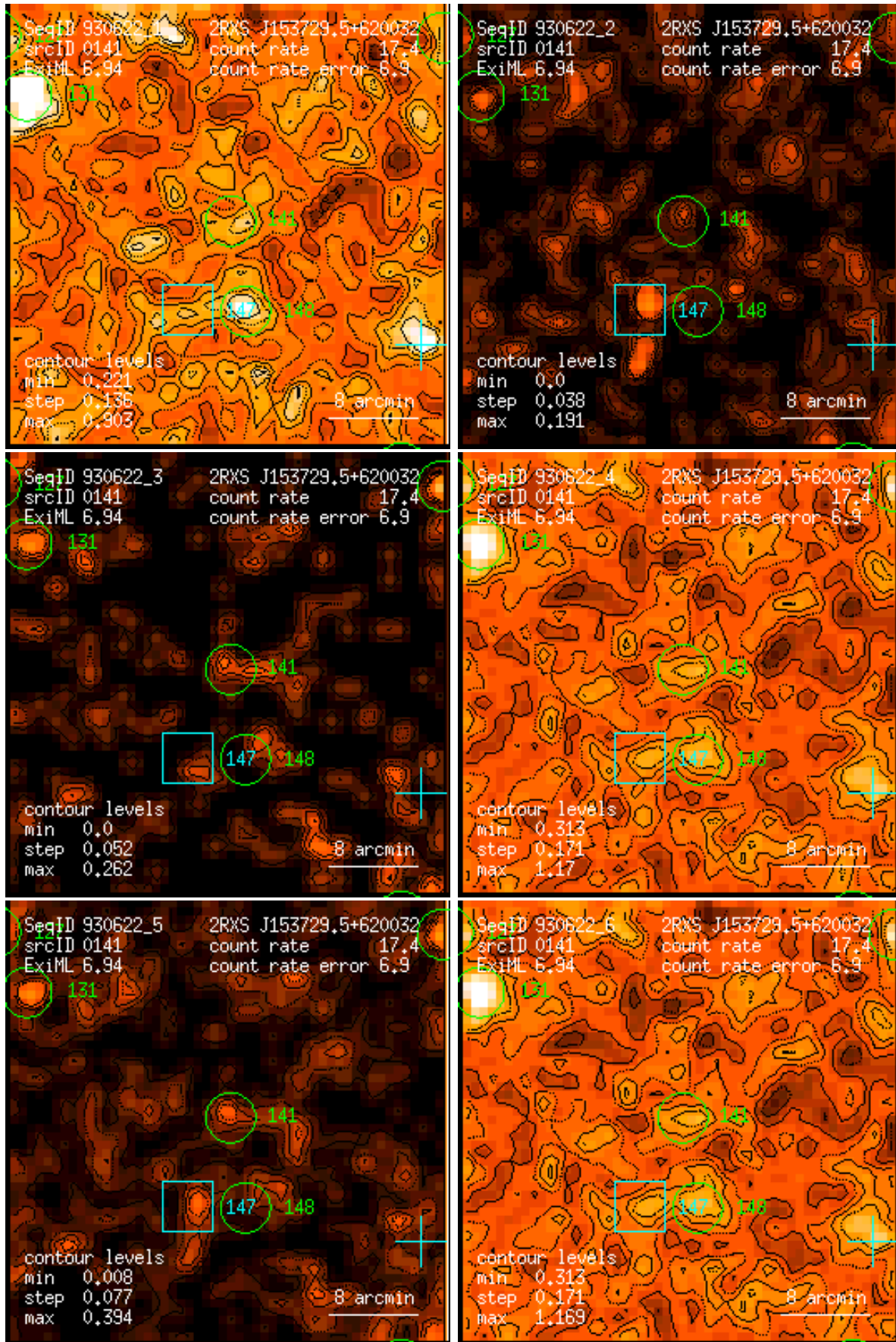
Figure 141: RASS 930622: detection 0141: band rate images, Gaussian filter: (1) PSPC channels 11 – 41, (2) 52 – 90, (3) 91 – 201, (4) 11 – 235, (5) 52 – 201, (6) 11 – 201. Broad band rates in counts/ks. Band rate contour levels in counts/ks/arcmin 2 .
