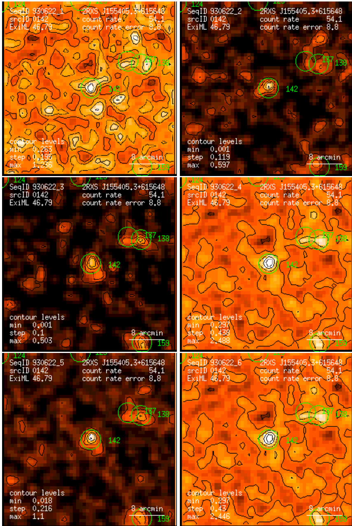
Figure 142: RASS 930622: detection 0142: band rate images, Gaussian filter: (1) PSPC channels 11 – 41, (2) 52 – 90, (3) 91 – 201, (4) 11 – 235, (5) 52 – 201, (6) 11 – 201. Broad band rates in counts/ks. Band rate contour levels in counts/ks/arcmin 2 .
