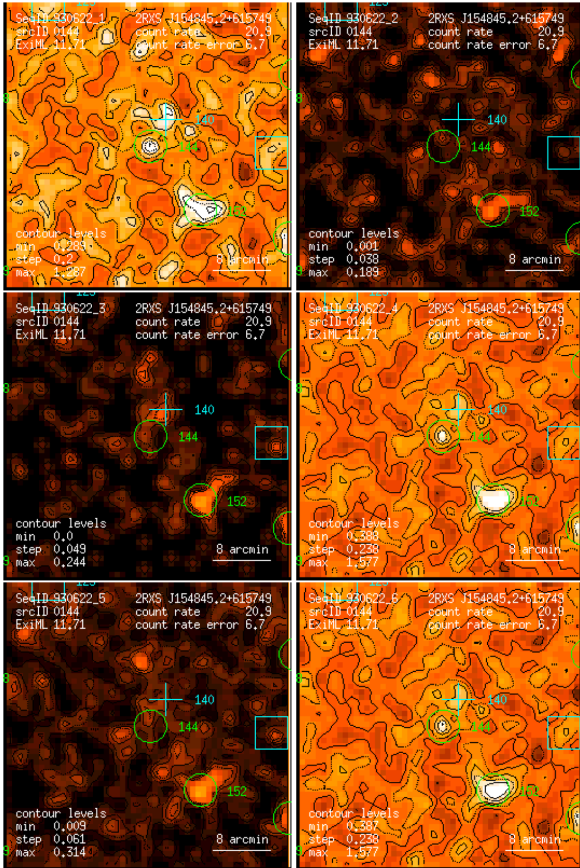
Figure 144: RASS 930622: detection 0144: band rate images, Gaussian filter: (1) PSPC channels 11 – 41, (2) 52 – 90, (3) 91 – 201, (4) 11 – 235, (5) 52 – 201, (6) 11 – 201. Broad band rates in counts/ks. Band rate contour levels in counts/ks/arcmin 2 .
