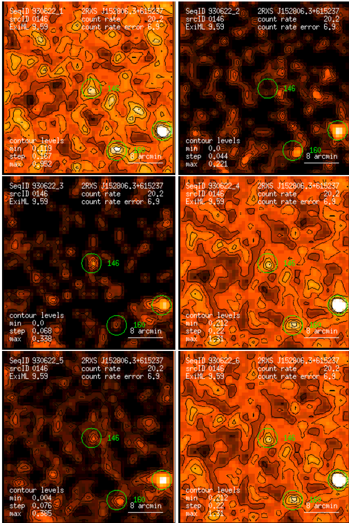
Figure 146: RASS 930622: detection 0146: band rate images, Gaussian filter: (1) PSPC channels 11 – 41, (2) 52 – 90, (3) 91 – 201, (4) 11 – 235, (5) 52 – 201, (6) 11 – 201. Broad band rates in counts/ks. Band rate contour levels in counts/ks/arcmin 2 .
