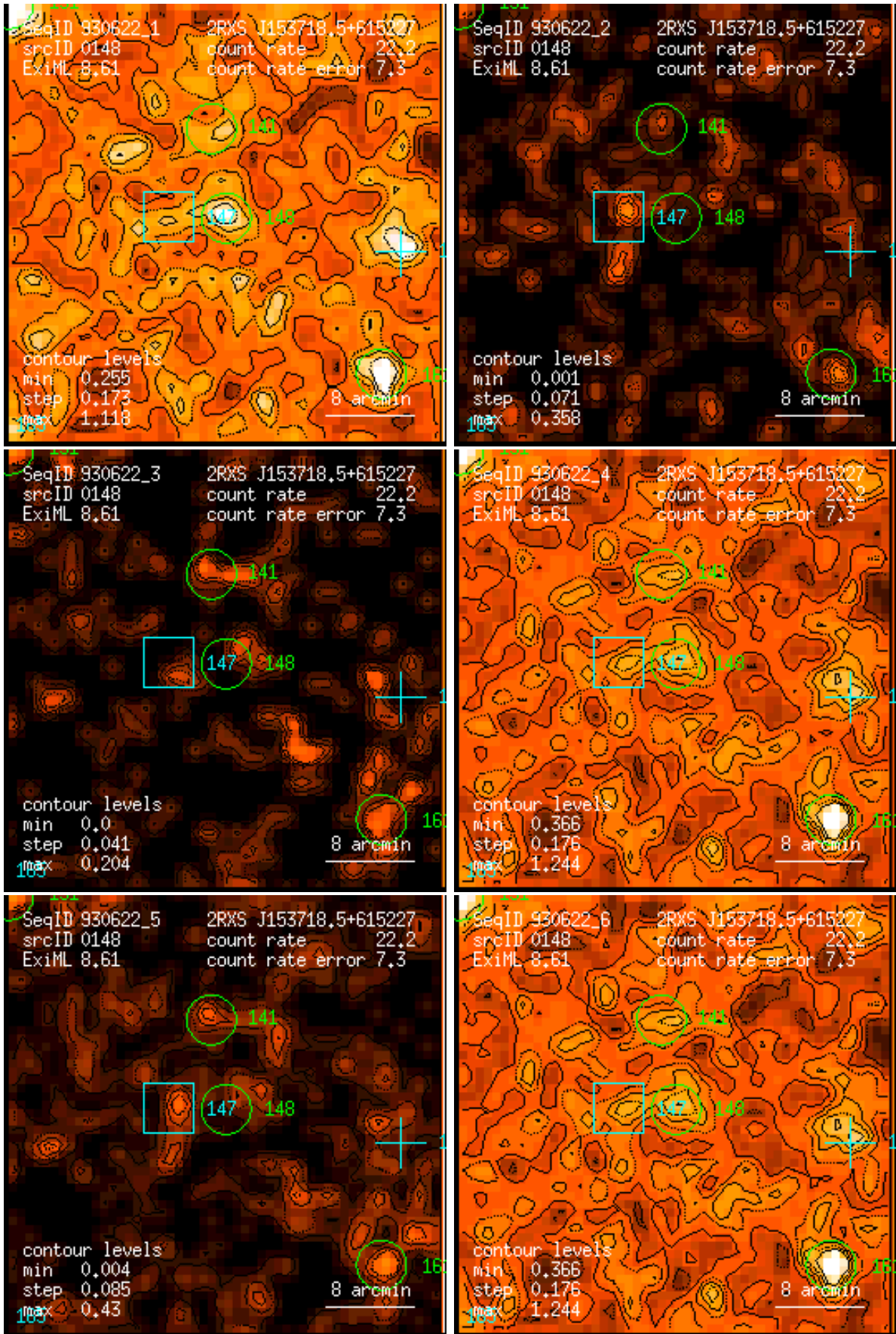
Figure 148: RASS 930622: detection 0148: band rate images, Gaussian filter: (1) PSPC channels 11 – 41, (2) 52 – 90, (3) 91 – 201, (4) 11 – 235, (5) 52 – 201, (6) 11 – 201. Broad band rates in counts/ks. Band rate contour levels in counts/ks/arcmin 2 .
