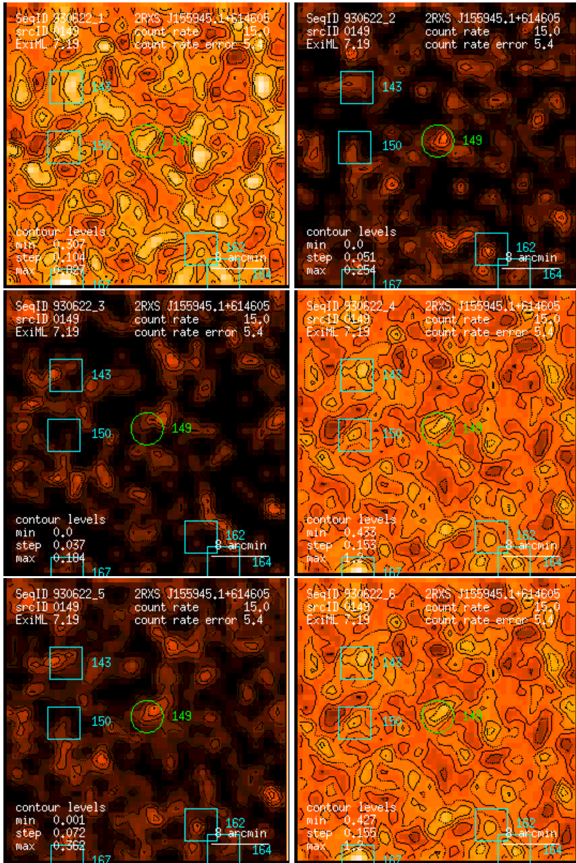
Figure 149: RASS 930622: detection 0149: band rate images, Gaussian filter: (1) PSPC channels 11 – 41, (2) 52 – 90, (3) 91 – 201, (4) 11 – 235, (5) 52 – 201, (6) 11 – 201. Broad band rates in counts/ks. Band rate contour levels in counts/ks/arcmin 2 .
