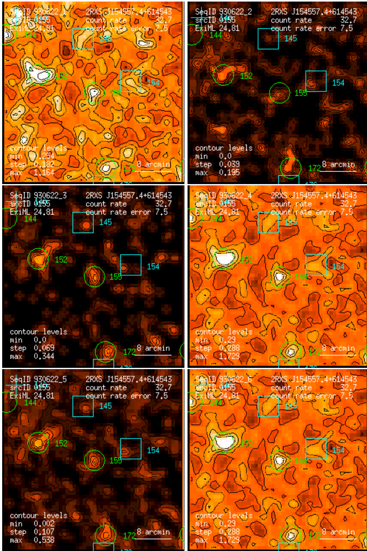
Figure 155: RASS 930622: detection 0155: band rate images, Gaussian filter: (1) PSPC channels 11 – 41, (2) 52 – 90, (3) 91 – 201, (4) 11 – 235, (5) 52 – 201, (6) 11 – 201. Broad band rates in counts/ks. Band rate contour levels in counts/ks/arcmin 2 .
