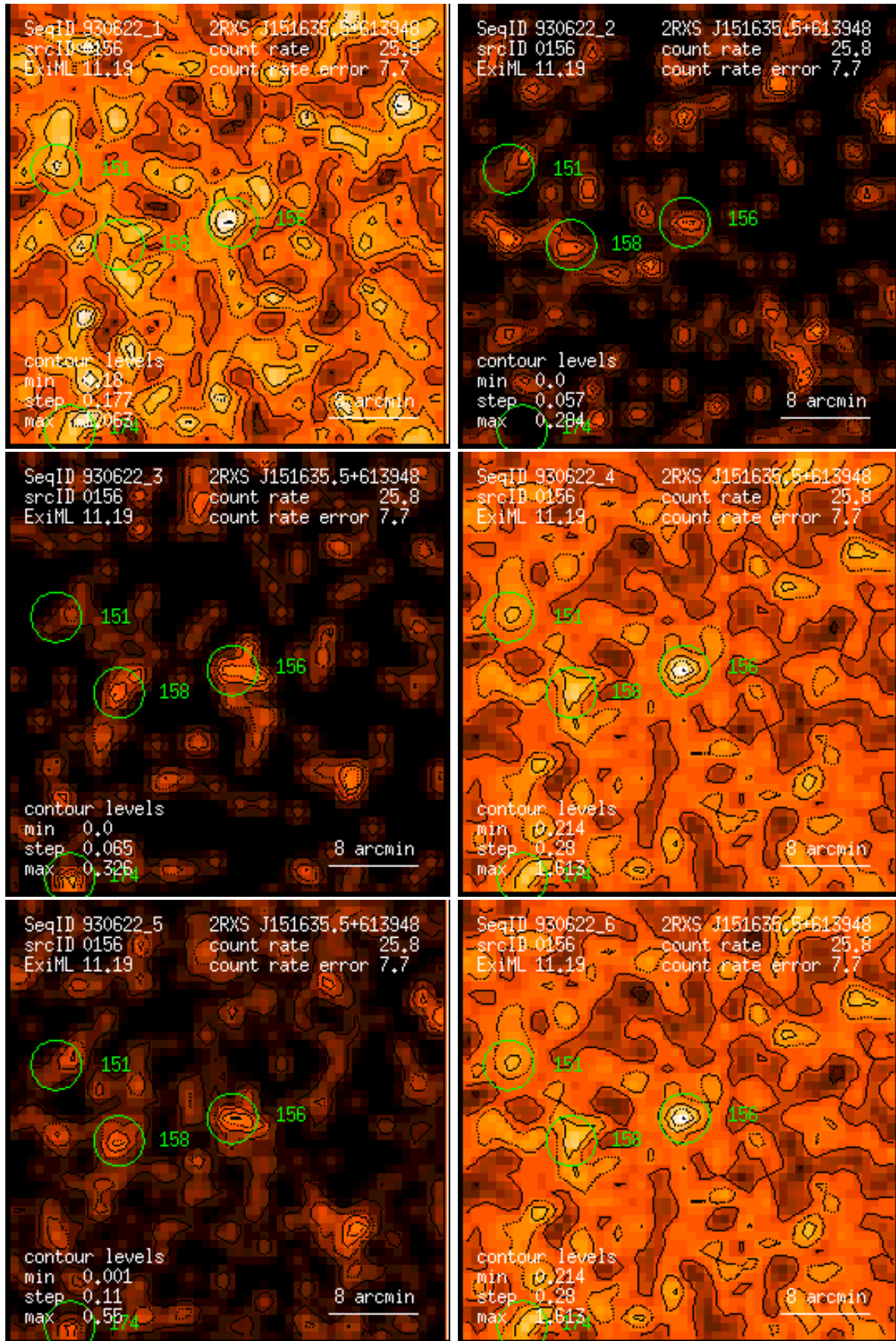
Figure 156: RASS 930622: detection 0156: band rate images, Gaussian filter: (1) PSPC channels 11 – 41, (2) 52 – 90, (3) 91 – 201, (4) 11 – 235, (5) 52 – 201, (6) 11 – 201. Broad band rates in counts/ks. Band rate contour levels in counts/ks/arcmin 2 .
