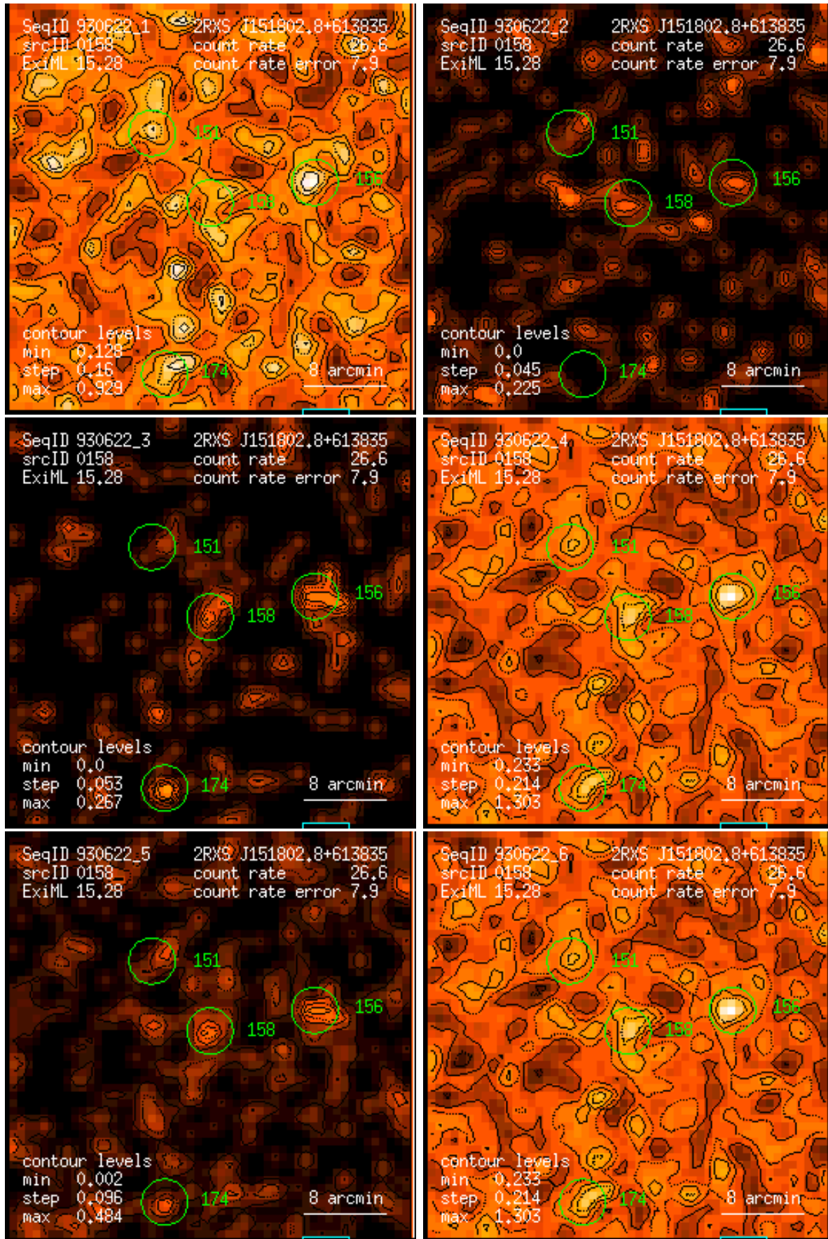
Figure 158: RASS 930622: detection 0158: band rate images, Gaussian filter: (1) PSPC channels 11 – 41, (2) 52 – 90, (3) 91 – 201, (4) 11 – 235, (5) 52 – 201, (6) 11 – 201. Broad band rates in counts/ks. Band rate contour levels in counts/ks/arcmin 2 .
