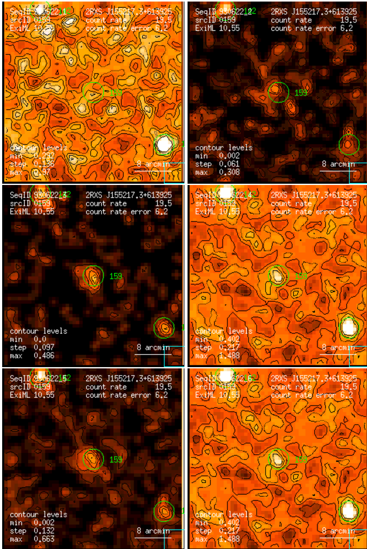
Figure 159: RASS 930622: detection 0159: band rate images, Gaussian filter: (1) PSPC channels 11 – 41, (2) 52 – 90, (3) 91 – 201, (4) 11 – 235, (5) 52 – 201, (6) 11 – 201. Broad band rates in counts/ks. Band rate contour levels in counts/ks/arcmin 2 .
