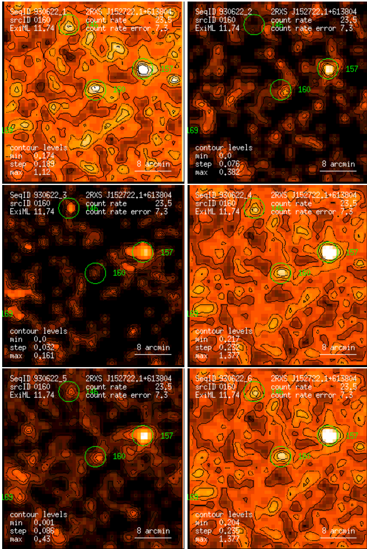
Figure 160: RASS 930622: detection 0160: band rate images, Gaussian filter: (1) PSPC channels 11 – 41, (2) 52 – 90, (3) 91 – 201, (4) 11 – 235, (5) 52 – 201, (6) 11 – 201. Broad band rates in counts/ks. Band rate contour levels in counts/ks/arcmin 2 .
