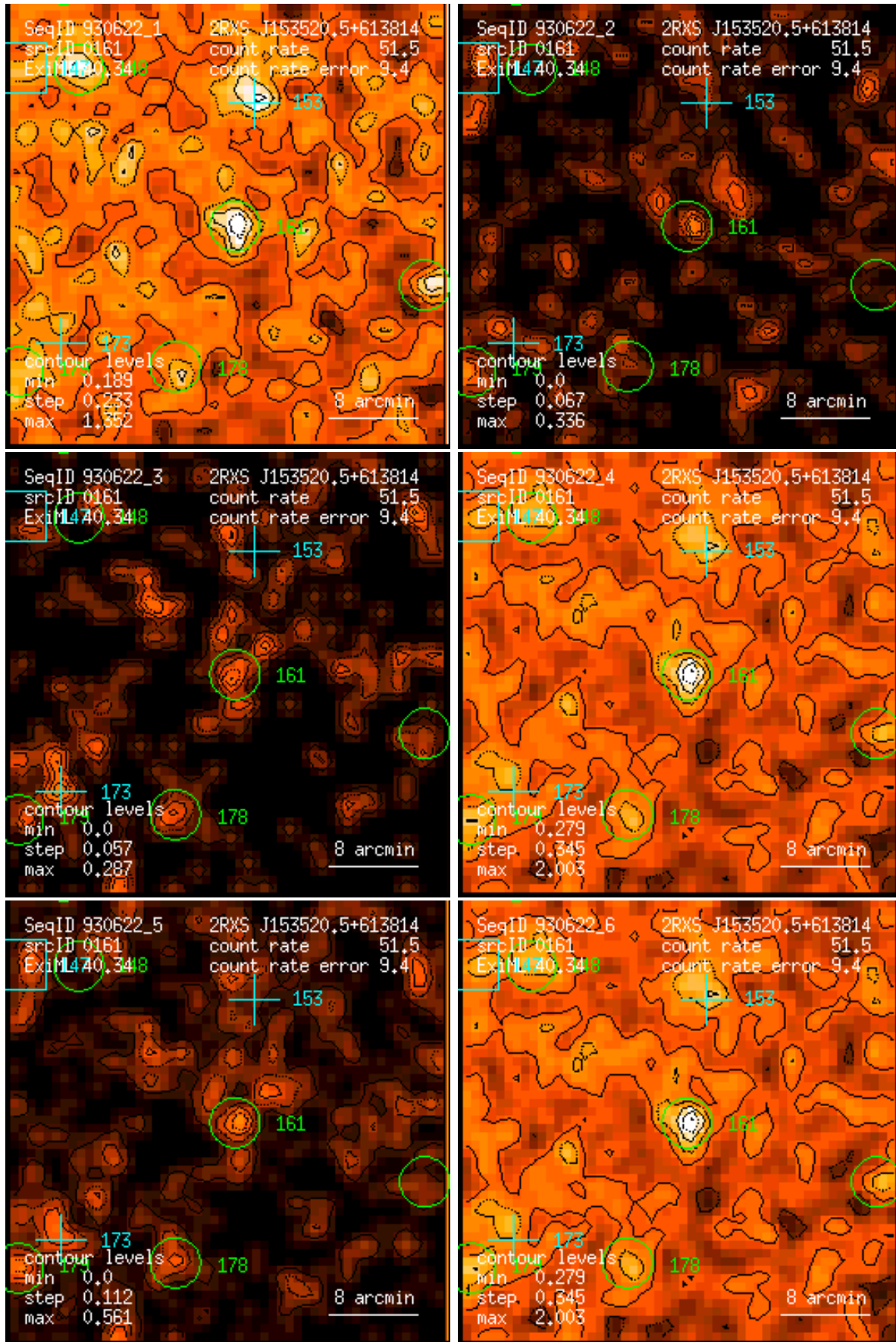
Figure 161: RASS 930622: detection 0161: band rate images, Gaussian filter: (1) PSPC channels 11 – 41, (2) 52 – 90, (3) 91 – 201, (4) 11 – 235, (5) 52 – 201, (6) 11 – 201. Broad band rates in counts/ks. Band rate contour levels in counts/ks/arcmin 2 .
