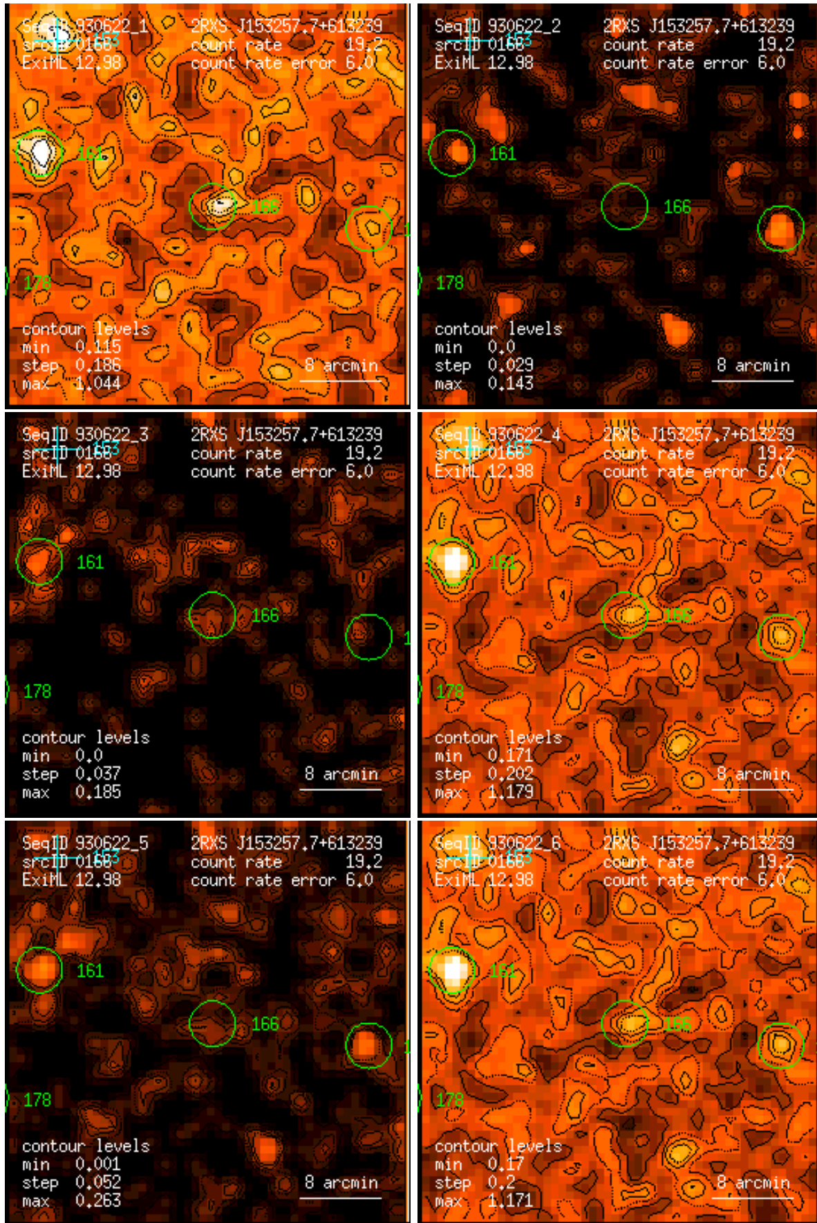
Figure 166: RASS 930622: detection 0166: band rate images, Gaussian filter: (1) PSPC channels 11 – 41, (2) 52 – 90, (3) 91 – 201, (4) 11 – 235, (5) 52 – 201, (6) 11 – 201. Broad band rates in counts/ks. Band rate contour levels in counts/ks/arcmin 2 .
