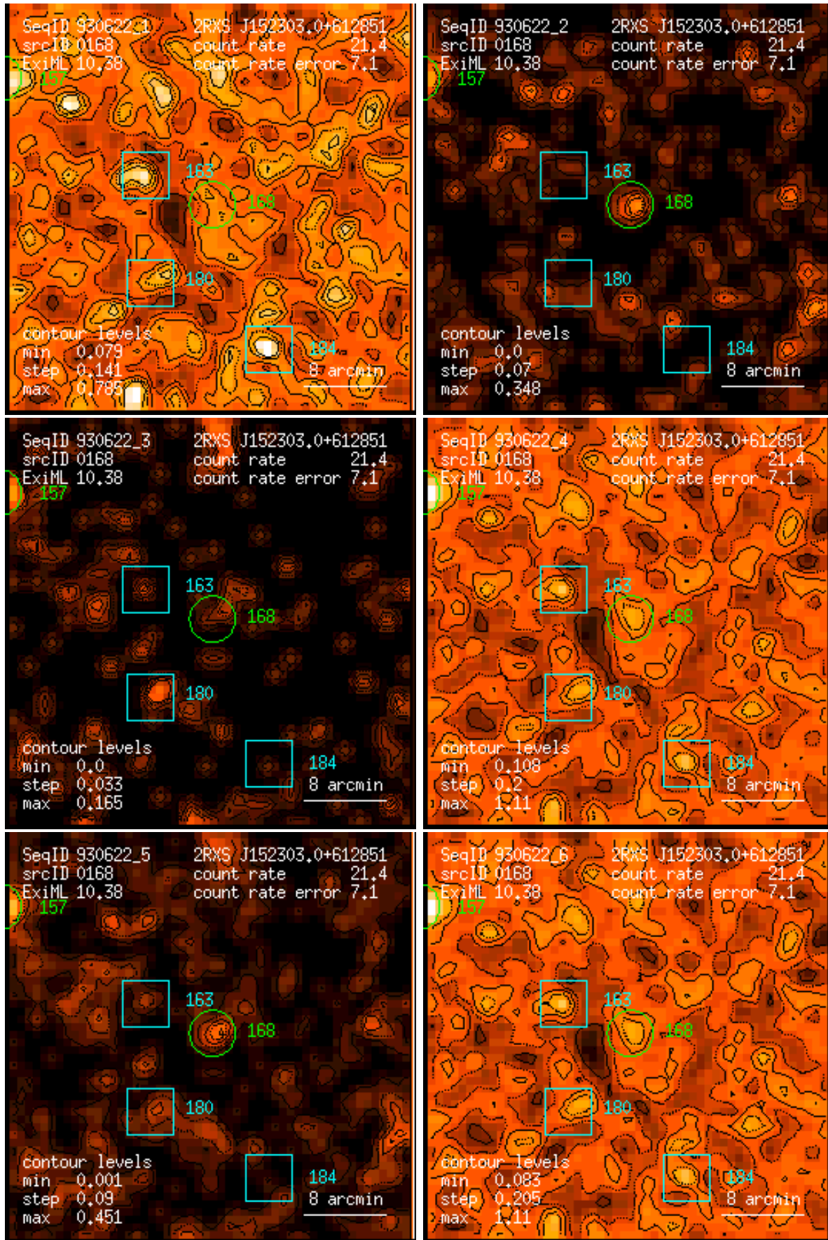
Figure 168: RASS 930622: detection 0168: band rate images, Gaussian filter: (1) PSPC channels 11 – 41, (2) 52 – 90, (3) 91 – 201, (4) 11 – 235, (5) 52 – 201, (6) 11 – 201. Broad band rates in counts/ks. Band rate contour levels in counts/ks/arcmin 2 .
