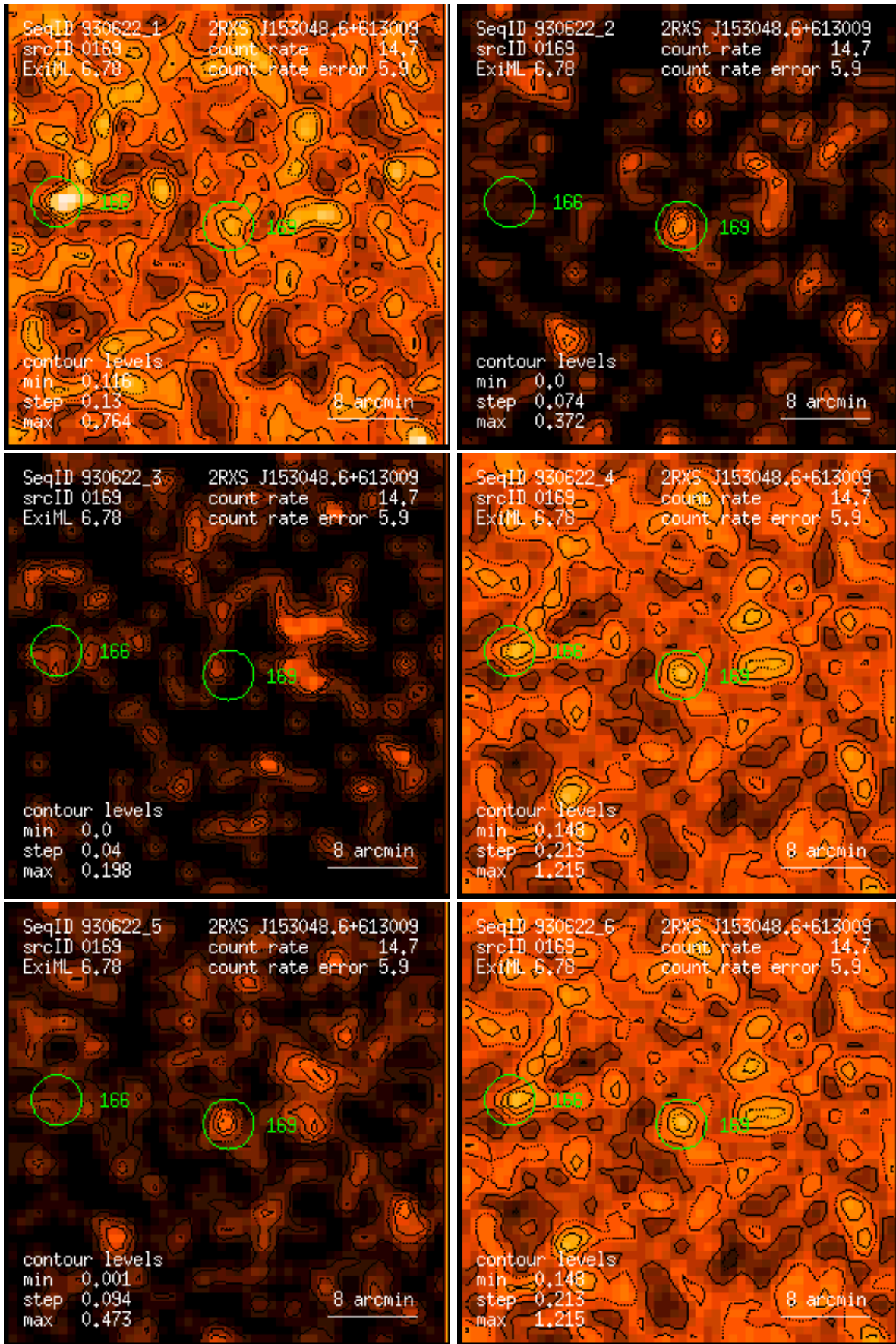
Figure 169: RASS 930622: detection 0169: band rate images, Gaussian filter: (1) PSPC channels 11 – 41, (2) 52 – 90, (3) 91 – 201, (4) 11 – 235, (5) 52 – 201, (6) 11 – 201. Broad band rates in counts/ks. Band rate contour levels in counts/ks/arcmin 2 .
