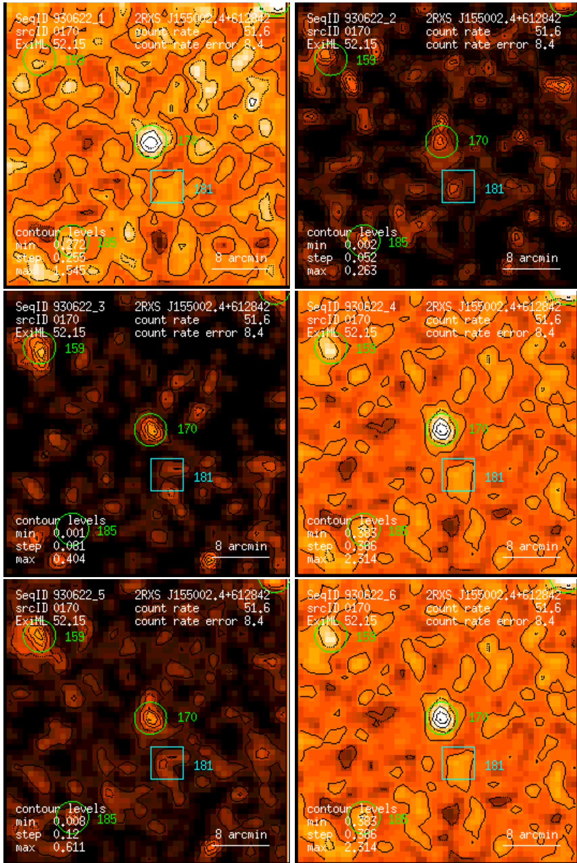
Figure 170: RASS 930622: detection 0170: band rate images, Gaussian filter: (1) PSPC channels 11 – 41, (2) 52 – 90, (3) 91 – 201, (4) 11 – 235, (5) 52 – 201, (6) 11 – 201. Broad band rates in counts/ks. Band rate contour levels in counts/ks/arcmin 2 .
