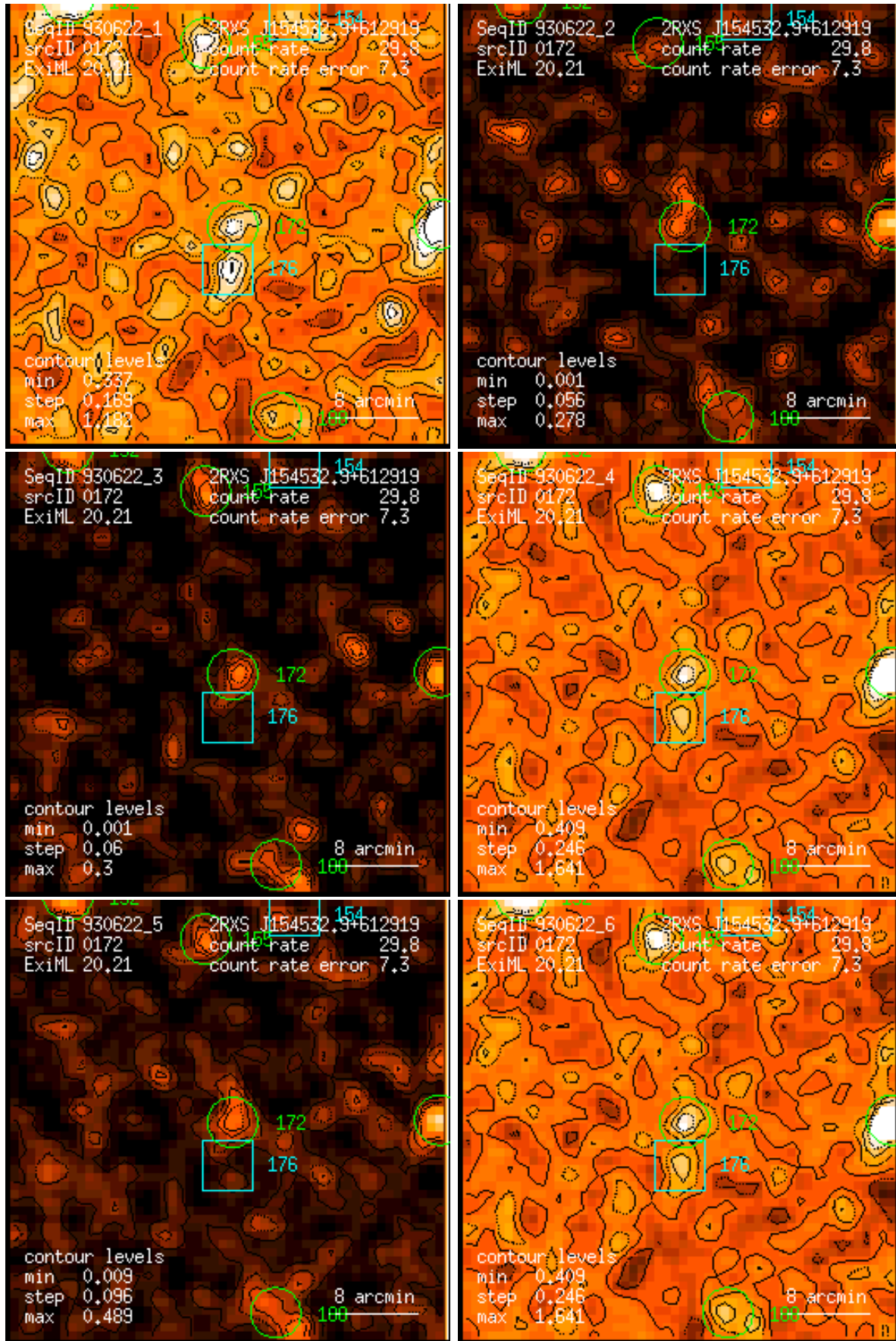
Figure 172: RASS 930622: detection 0172: band rate images, Gaussian filter: (1) PSPC channels 11 – 41, (2) 52 – 90, (3) 91 – 201, (4) 11 – 235, (5) 52 – 201, (6) 11 – 201. Broad band rates in counts/ks. Band rate contour levels in counts/ks/arcmin 2 .
