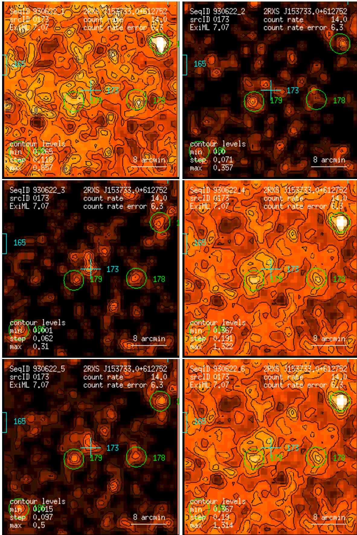
Figure 173: RASS 930622: detection 0173: band rate images, Gaussian filter: (1) PSPC channels 11 – 41, (2) 52 – 90, (3) 91 – 201, (4) 11 – 235, (5) 52 – 201, (6) 11 – 201. Broad band rates in counts/ks. Band rate contour levels in counts/ks/arcmin 2 .
