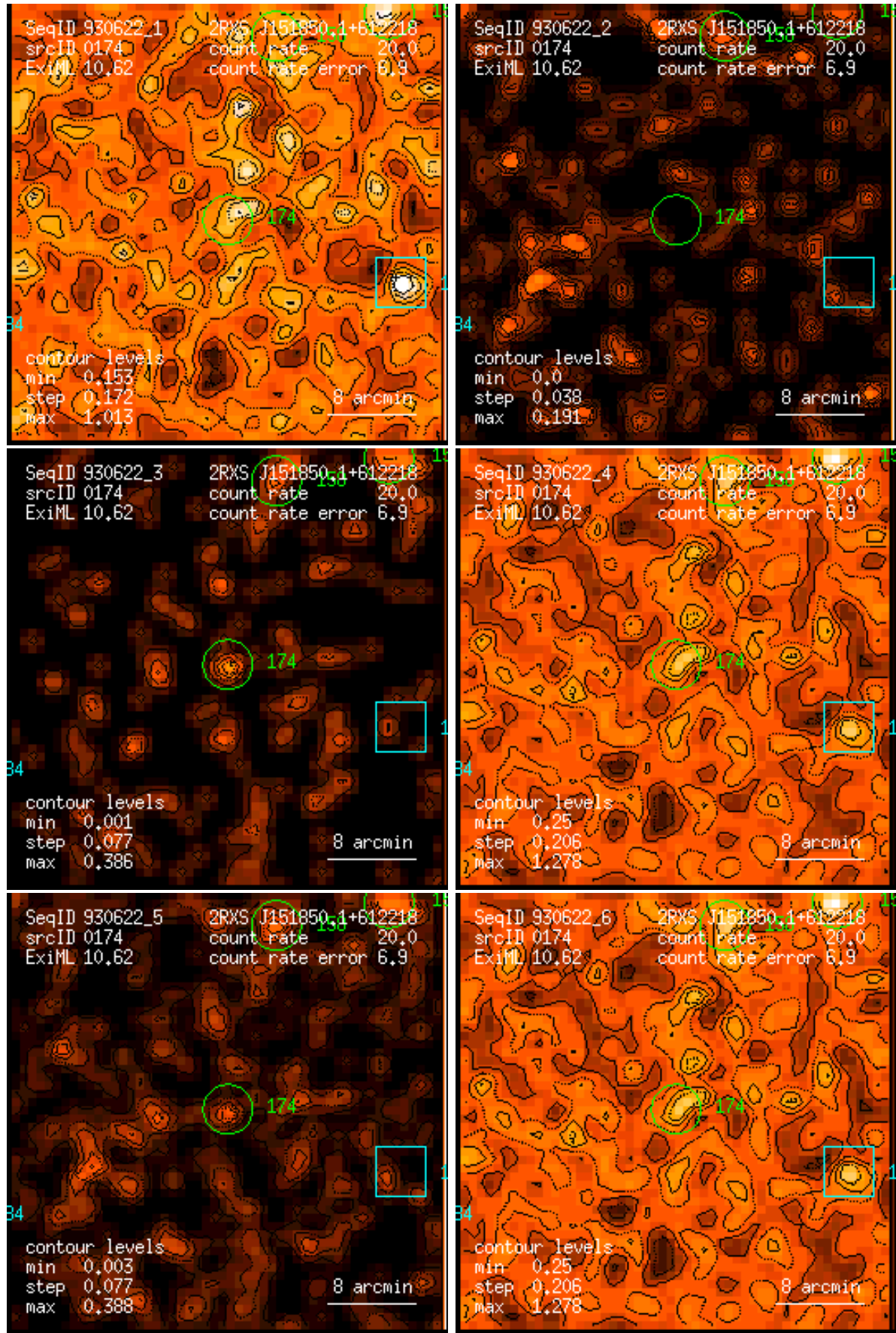
Figure 174: RASS 930622: detection 0174: band rate images, Gaussian filter: (1) PSPC channels 11 – 41, (2) 52 – 90, (3) 91 – 201, (4) 11 – 235, (5) 52 – 201, (6) 11 – 201. Broad band rates in counts/ks. Band rate contour levels in counts/ks/arcmin 2 .
