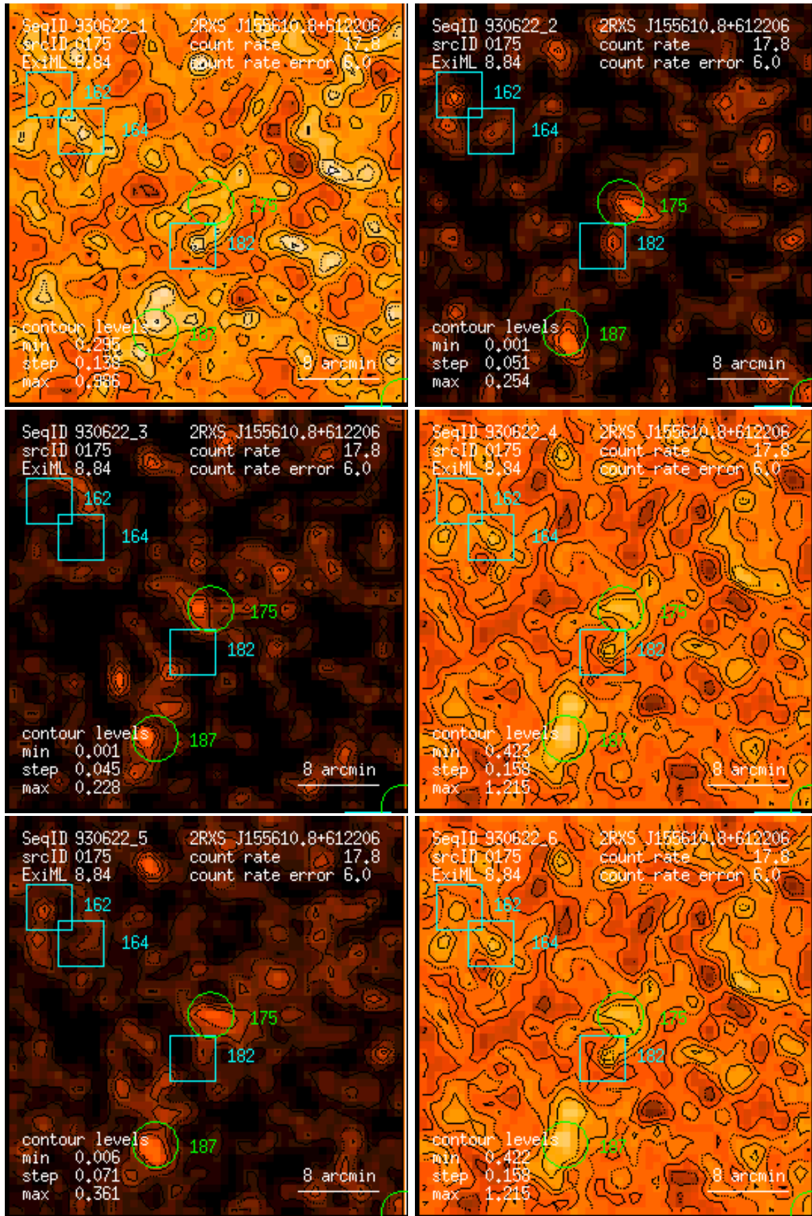
Figure 175: RASS 930622: detection 0175: band rate images, Gaussian filter: (1) PSPC channels 11 – 41, (2) 52 – 90, (3) 91 – 201, (4) 11 – 235, (5) 52 – 201, (6) 11 – 201. Broad band rates in counts/ks. Band rate contour levels in counts/ks/arcmin 2 .
