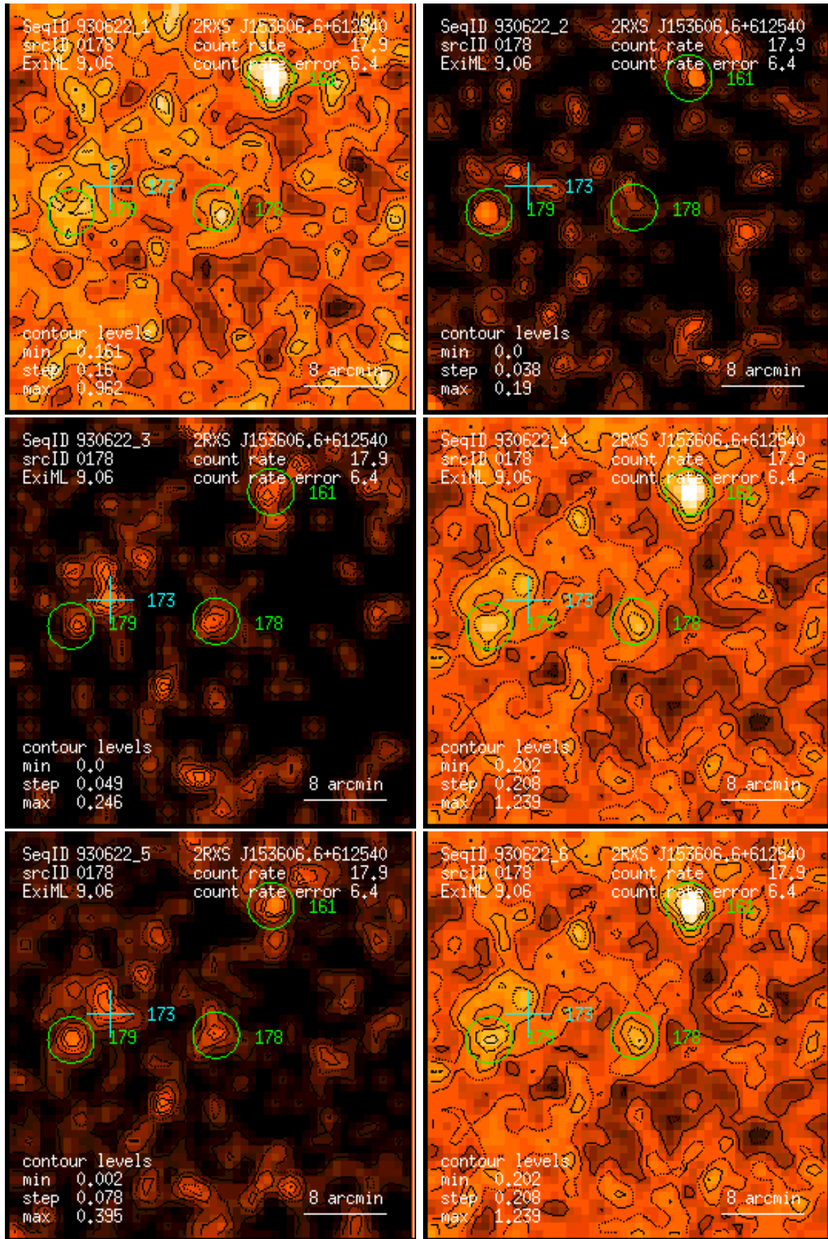
Figure 178: RASS 930622: detection 0178: band rate images, Gaussian filter: (1) PSPC channels 11 – 41, (2) 52 – 90, (3) 91 – 201, (4) 11 – 235, (5) 52 – 201, (6) 11 – 201. Broad band rates in counts/ks. Band rate contour levels in counts/ks/arcmin 2 .
