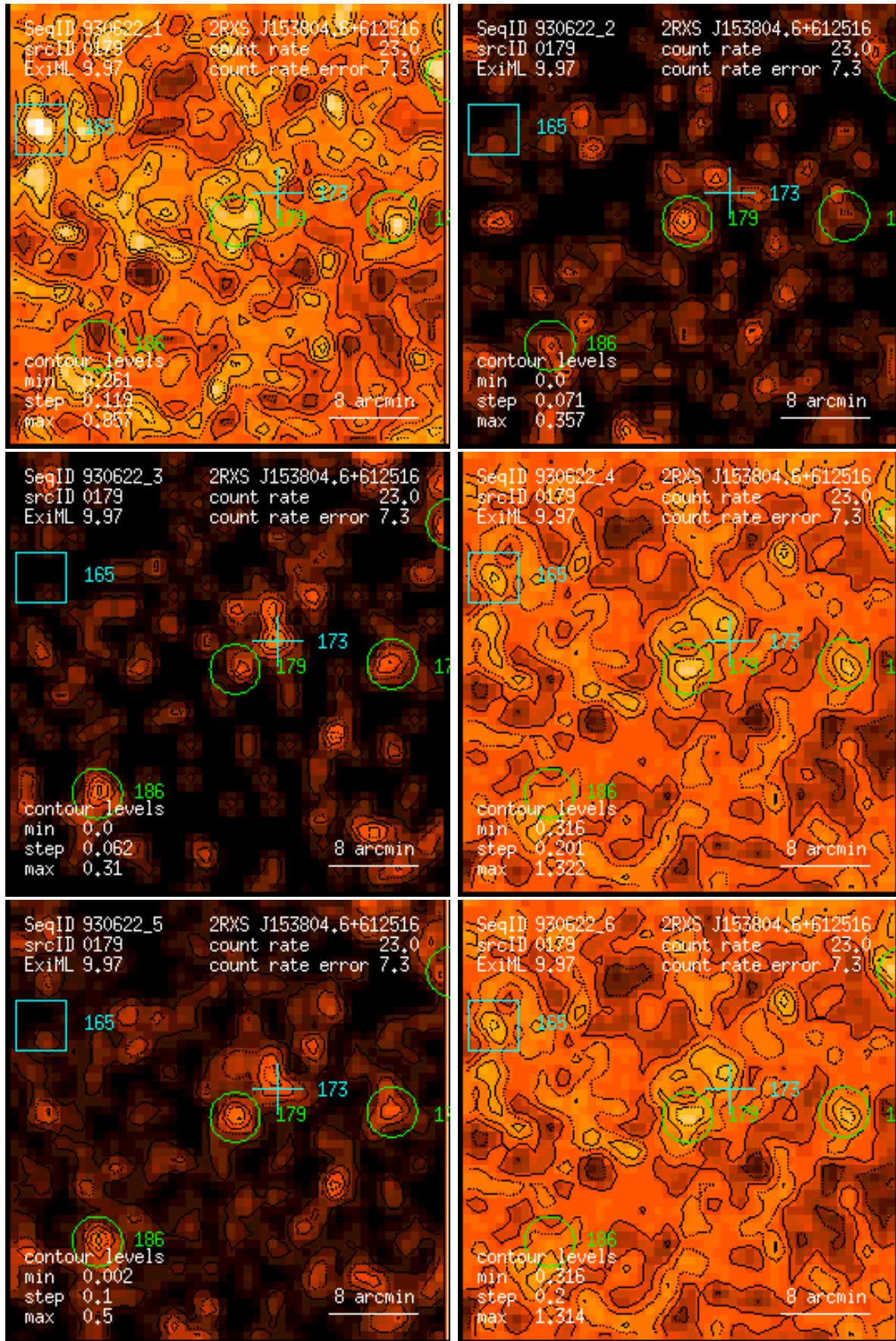
Figure 179: RASS 930622: detection 0179: band rate images, Gaussian filter: (1) PSPC channels 11 – 41, (2) 52 – 90, (3) 91 – 201, (4) 11 – 235, (5) 52 – 201, (6) 11 – 201. Broad band rates in counts/ks. Band rate contour levels in counts/ks/arcmin 2 .
