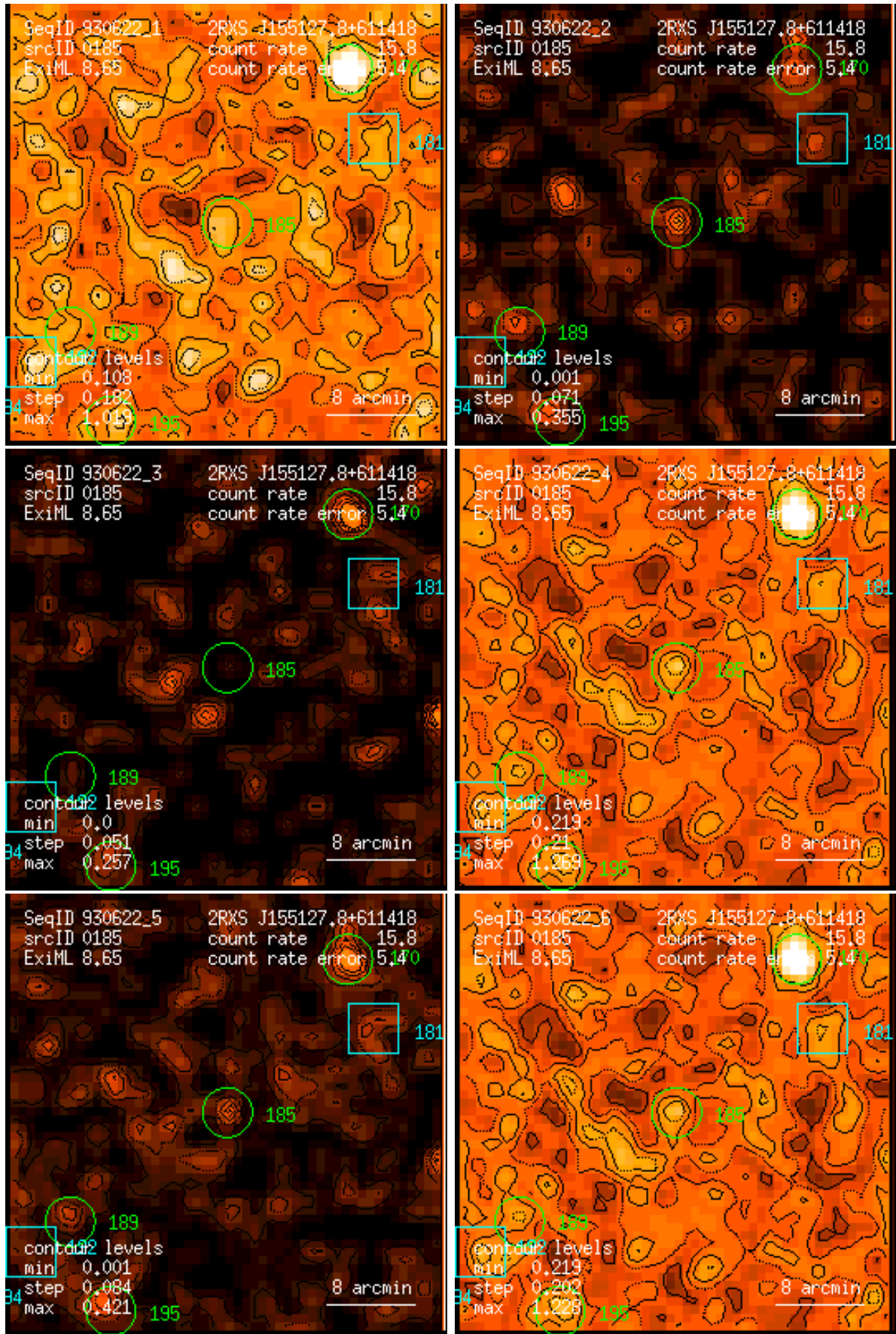
Figure 185: RASS 930622: detection 0185: band rate images, Gaussian filter: (1) PSPC channels 11 – 41, (2) 52 – 90, (3) 91 – 201, (4) 11 – 235, (5) 52 – 201, (6) 11 – 201. Broad band rates in counts/ks. Band rate contour levels in counts/ks/arcmin 2 .
