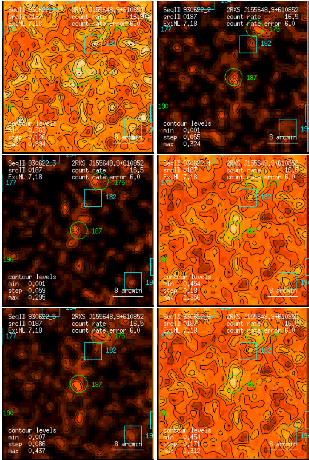
Figure 187: RASS 930622: detection 0187: band rate images, Gaussian filter: (1) PSPC channels 11 – 41, (2) 52 – 90, (3) 91 – 201, (4) 11 – 235, (5) 52 – 201, (6) 11 – 201. Broad band rates in counts/ks. Band rate contour levels in counts/ks/arcmin 2 .
