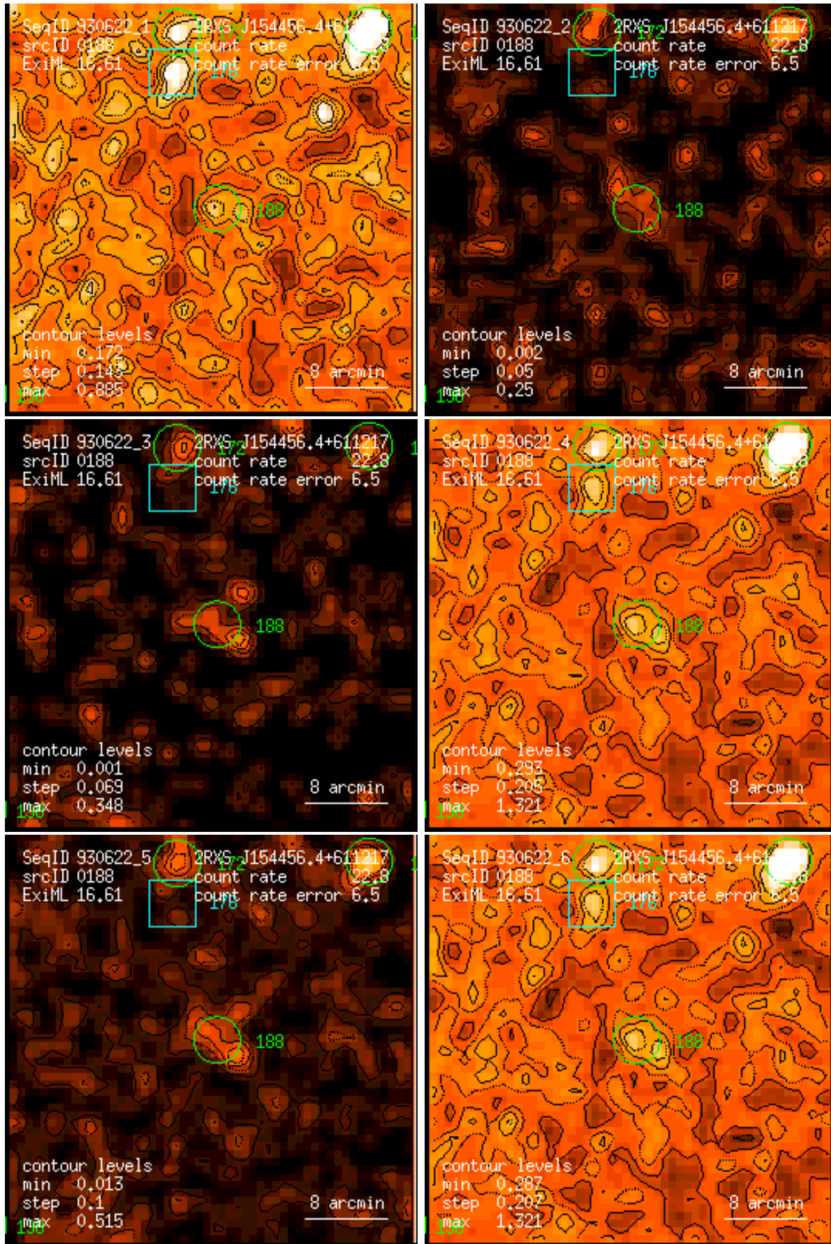
Figure 188: RASS 930622: detection 0188: band rate images, Gaussian filter: (1) PSPC channels 11 – 41, (2) 52 – 90, (3) 91 – 201, (4) 11 – 235, (5) 52 – 201, (6) 11 – 201. Broad band rates in counts/ks. Band rate contour levels in counts/ks/arcmin 2 .
