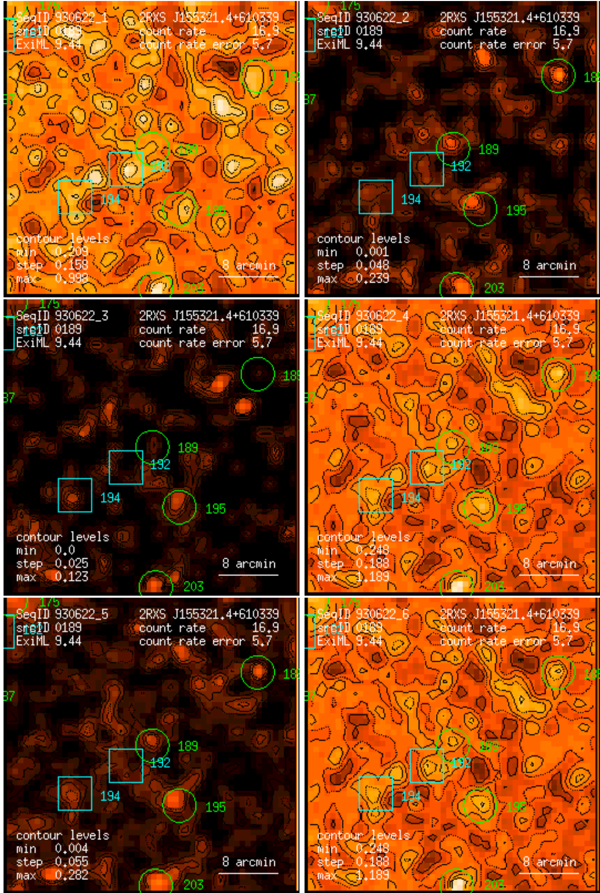
Figure 189: RASS 930622: detection 0189: band rate images, Gaussian filter: (1) PSPC channels 11 – 41, (2) 52 – 90, (3) 91 – 201, (4) 11 – 235, (5) 52 – 201, (6) 11 – 201. Broad band rates in counts/ks. Band rate contour levels in counts/ks/arcmin 2 .
