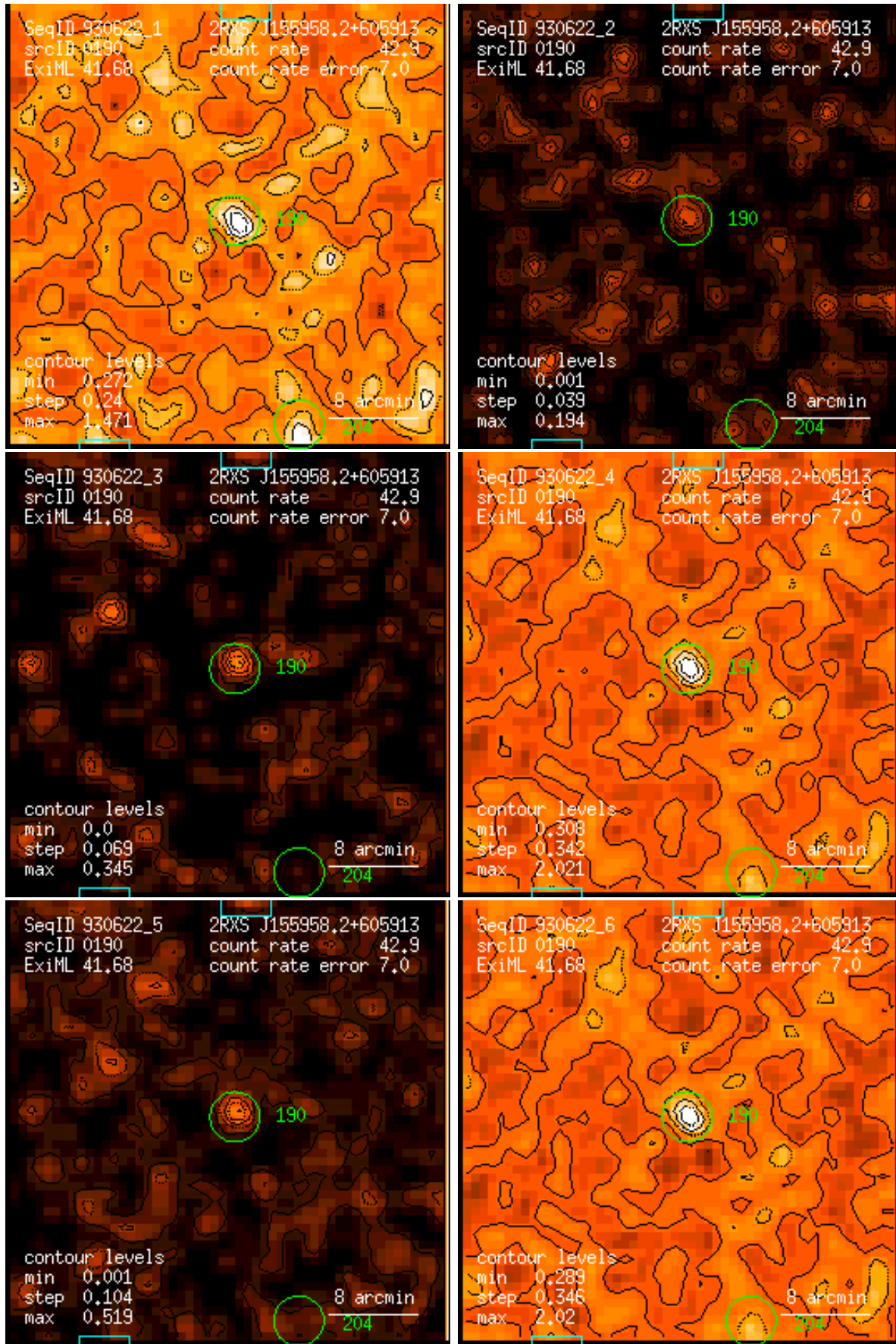
Figure 190: RASS 930622: detection 0190: band rate images, Gaussian filter: (1) PSPC channels 11 – 41, (2) 52 – 90, (3) 91 – 201, (4) 11 – 235, (5) 52 – 201, (6) 11 – 201. Broad band rates in counts/ks. Band rate contour levels in counts/ks/arcmin 2 .
