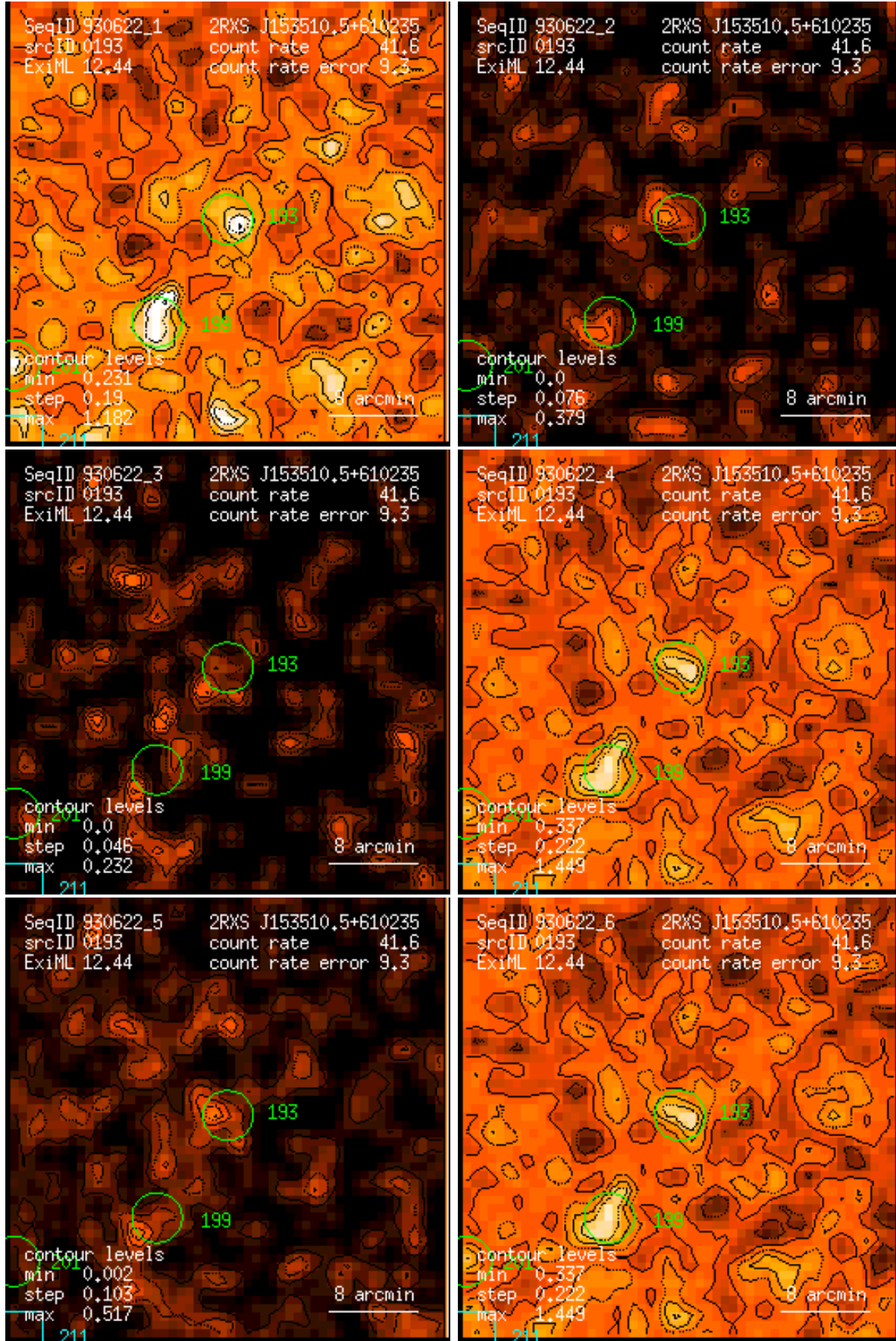
Figure 193: RASS 930622: detection 0193: band rate images, Gaussian filter: (1) PSPC channels 11 – 41, (2) 52 – 90, (3) 91 – 201, (4) 11 – 235, (5) 52 – 201, (6) 11 – 201. Broad band rates in counts/ks. Band rate contour levels in counts/ks/arcmin 2 .
