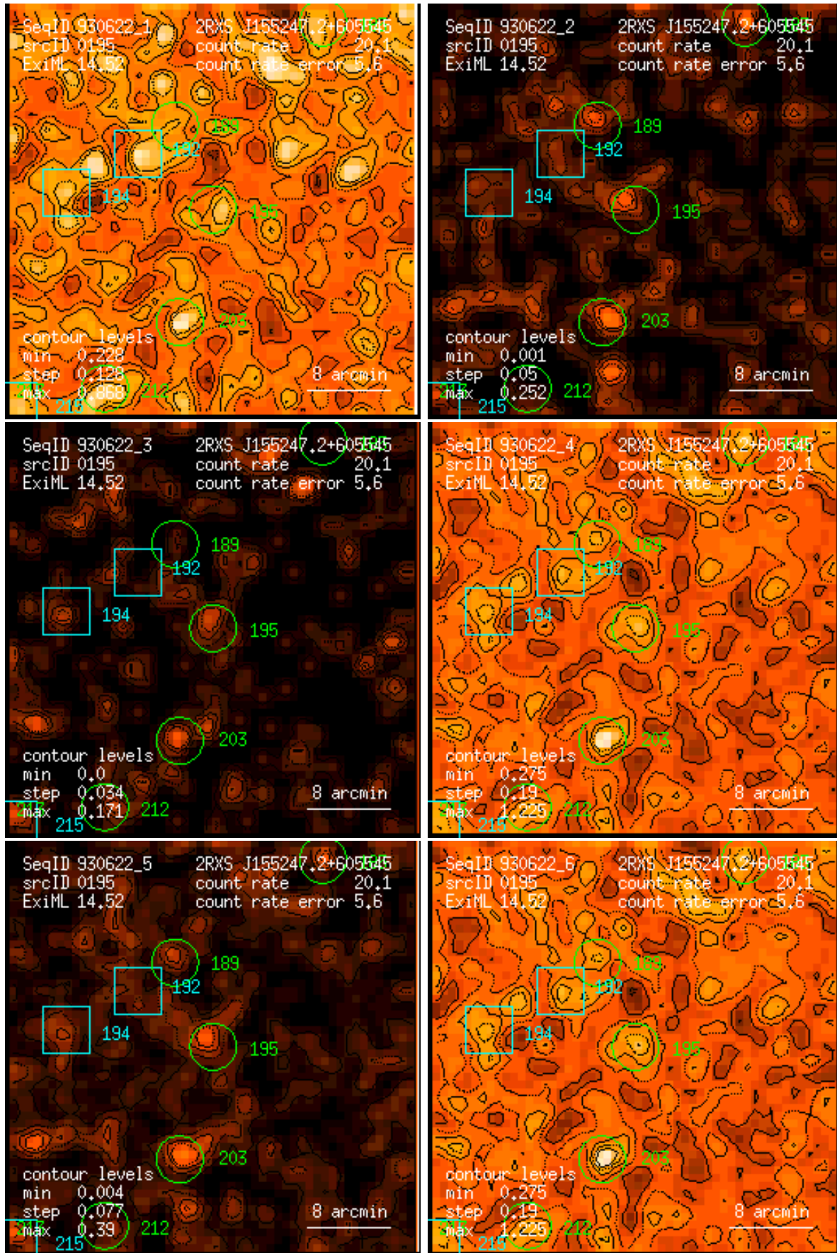
Figure 195: RASS 930622: detection 0195: band rate images, Gaussian filter: (1) PSPC channels 11 – 41, (2) 52 – 90, (3) 91 – 201, (4) 11 – 235, (5) 52 – 201, (6) 11 – 201. Broad band rates in counts/ks. Band rate contour levels in counts/ks/arcmin 2 .
