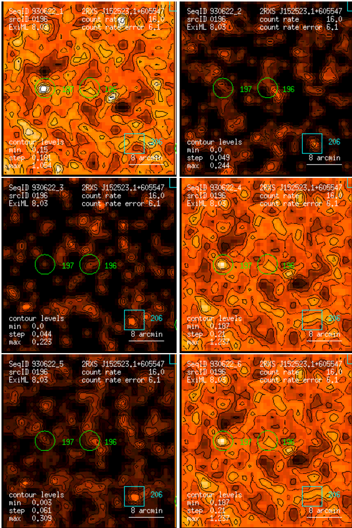
Figure 196: RASS 930622: detection 0196: band rate images, Gaussian filter: (1) PSPC channels 11 – 41, (2) 52 – 90, (3) 91 – 201, (4) 11 – 235, (5) 52 – 201, (6) 11 – 201. Broad band rates in counts/ks. Band rate contour levels in counts/ks/arcmin 2 .
