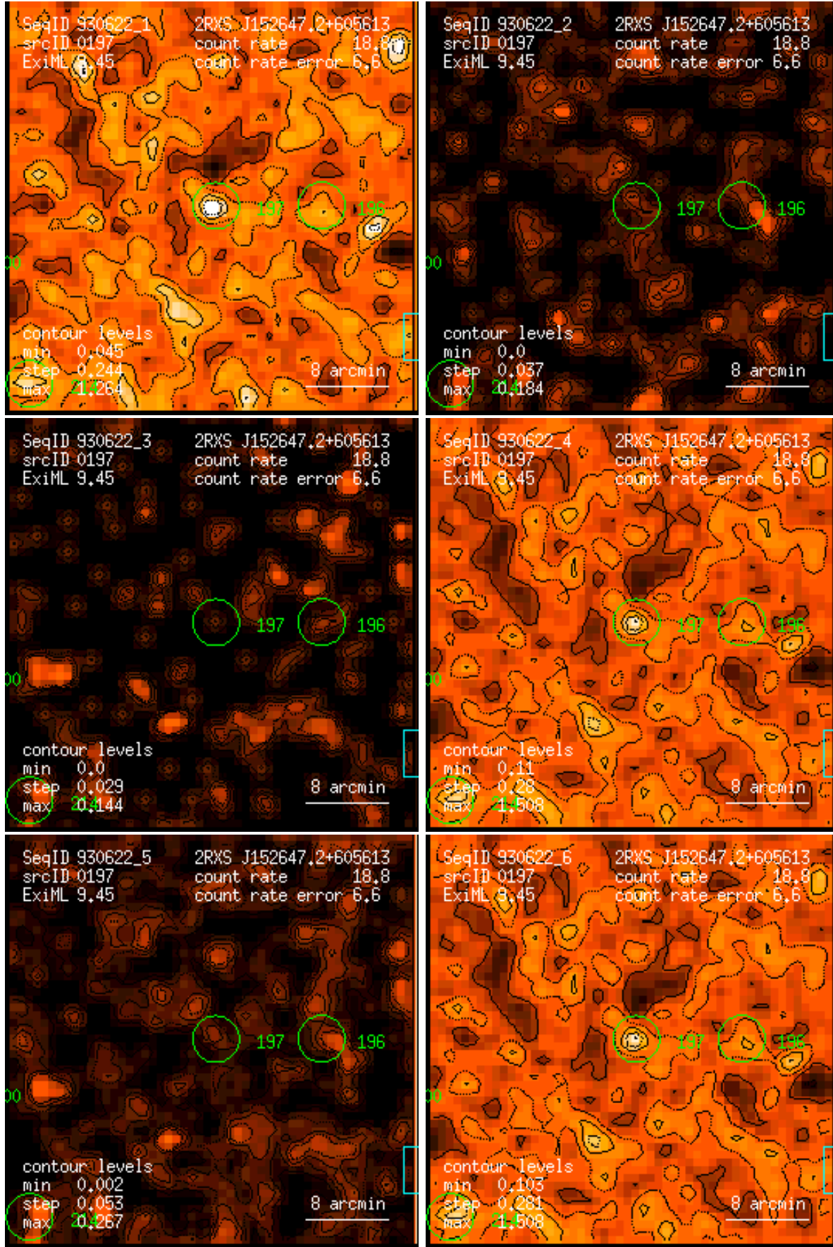
Figure 197: RASS 930622: detection 0197: band rate images, Gaussian filter: (1) PSPC channels 11 – 41, (2) 52 – 90, (3) 91 – 201, (4) 11 – 235, (5) 52 – 201, (6) 11 – 201. Broad band rates in counts/ks. Band rate contour levels in counts/ks/arcmin 2 .
