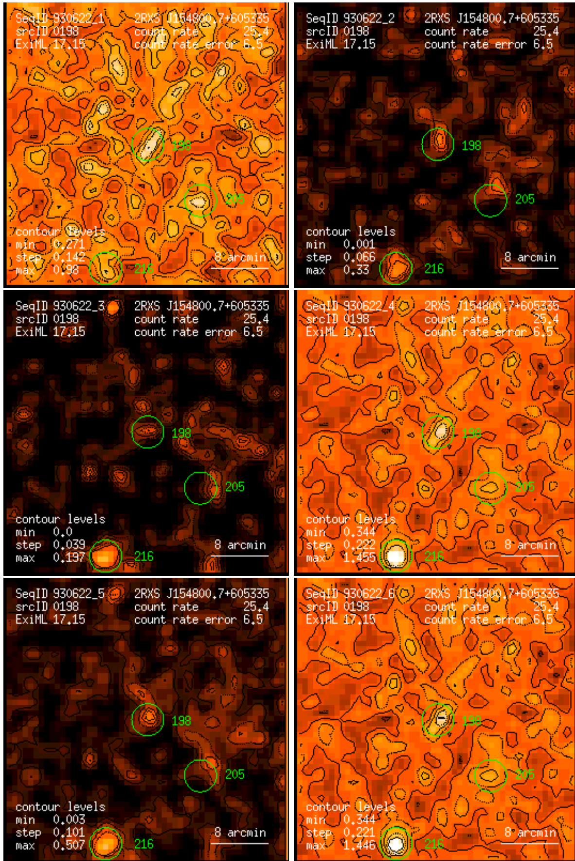
Figure 198: RASS 930622: detection 0198: band rate images, Gaussian filter: (1) PSPC channels 11 – 41, (2) 52 – 90, (3) 91 – 201, (4) 11 – 235, (5) 52 – 201, (6) 11 – 201. Broad band rates in counts/ks. Band rate contour levels in counts/ks/arcmin 2 .
