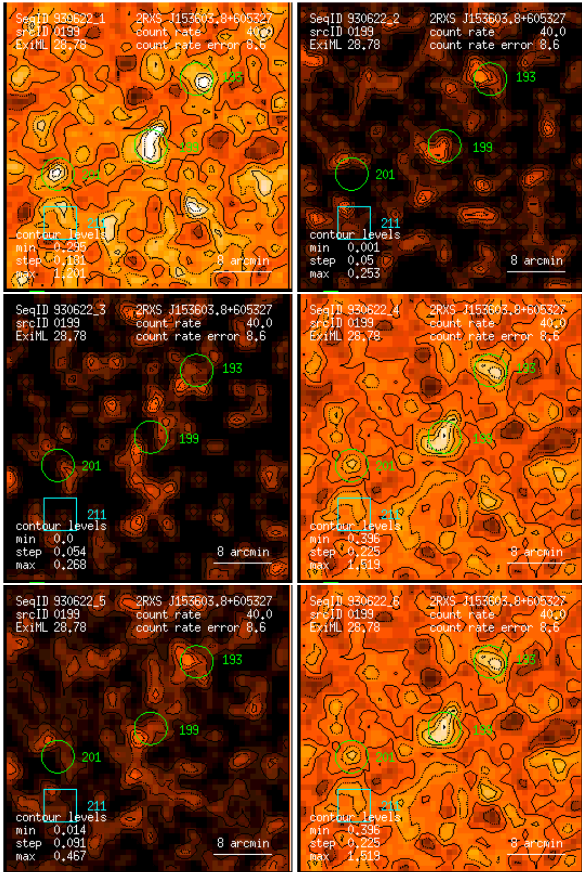
Figure 199: RASS 930622: detection 0199: band rate images, Gaussian filter: (1) PSPC channels 11 – 41, (2) 52 – 90, (3) 91 – 201, (4) 11 – 235, (5) 52 – 201, (6) 11 – 201. Broad band rates in counts/ks. Band rate contour levels in counts/ks/arcmin 2 .
