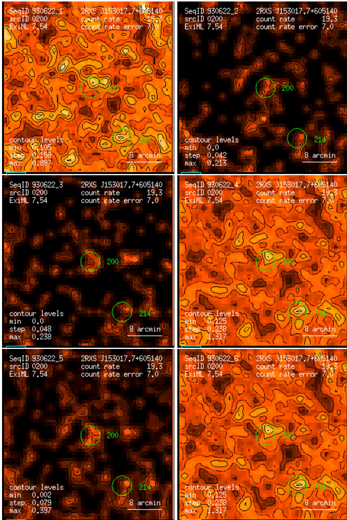
Figure 200: RASS 930622: detection 0200: band rate images, Gaussian filter: (1) PSPC channels 11 – 41, (2) 52 – 90, (3) 91 – 201, (4) 11 – 235, (5) 52 – 201, (6) 11 – 201. Broad band rates in counts/ks. Band rate contour levels in counts/ks/arcmin 2 .
