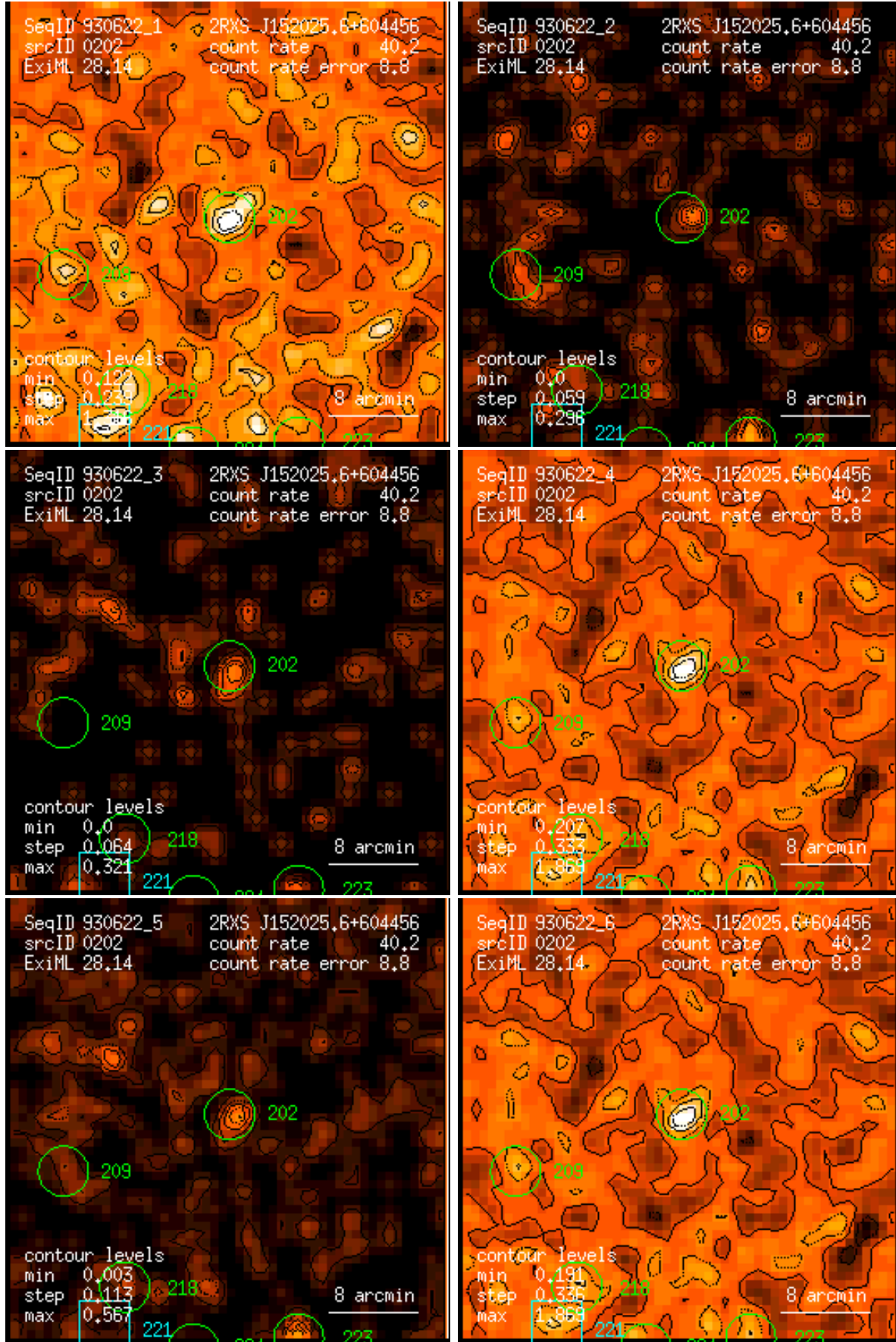
Figure 202: RASS 930622: detection 0202: band rate images, Gaussian filter: (1) PSPC channels 11 – 41, (2) 52 – 90, (3) 91 – 201, (4) 11 – 235, (5) 52 – 201, (6) 11 – 201. Broad band rates in counts/ks. Band rate contour levels in counts/ks/arcmin 2 .
