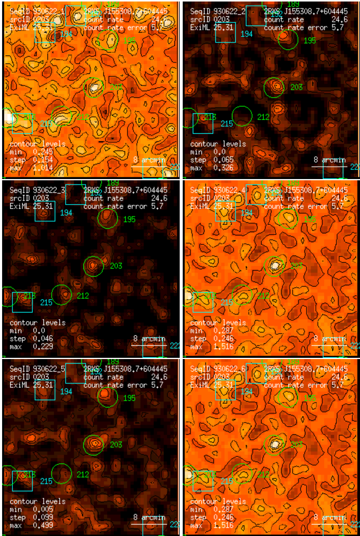
Figure 203: RASS 930622: detection 0203: band rate images, Gaussian filter: (1) PSPC channels 11 – 41, (2) 52 – 90, (3) 91 – 201, (4) 11 – 235, (5) 52 – 201, (6) 11 – 201. Broad band rates in counts/ks. Band rate contour levels in counts/ks/arcmin 2 .
