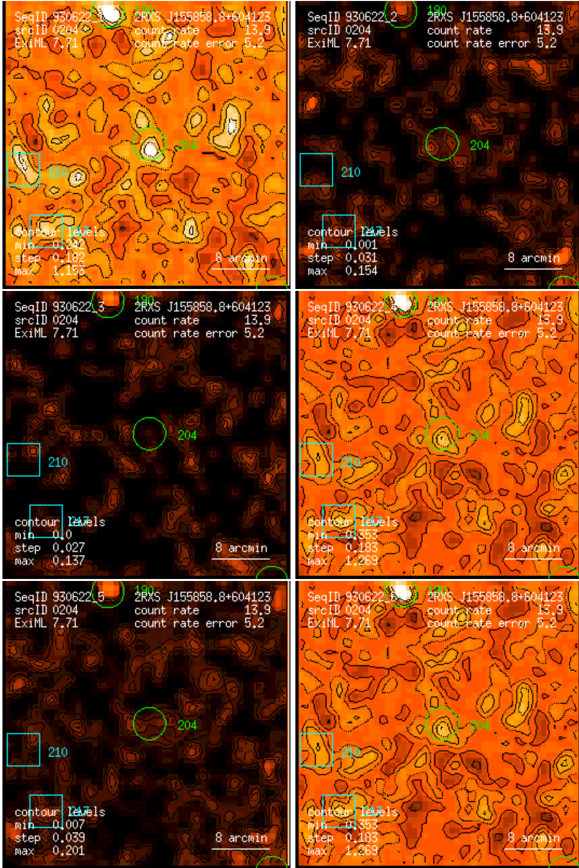
Figure 204: RASS 930622: detection 0204: band rate images, Gaussian filter: (1) PSPC channels 11 – 41, (2) 52 – 90, (3) 91 – 201, (4) 11 – 235, (5) 52 – 201, (6) 11 – 201. Broad band rates in counts/ks. Band rate contour levels in counts/ks/arcmin 2 .
