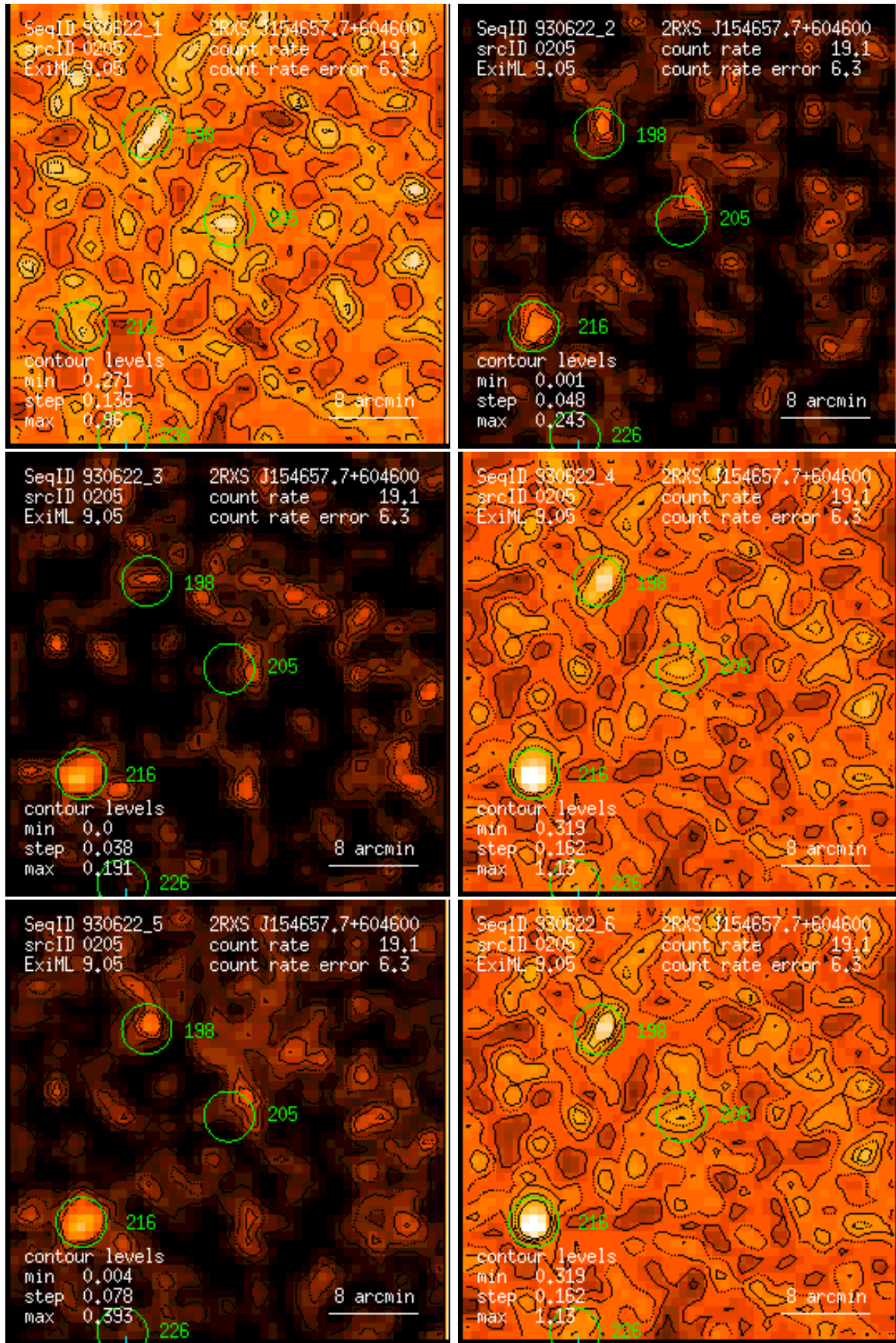
Figure 205: RASS 930622: detection 0205: band rate images, Gaussian filter: (1) PSPC channels 11 – 41, (2) 52 – 90, (3) 91 – 201, (4) 11 – 235, (5) 52 – 201, (6) 11 – 201. Broad band rates in counts/ks. Band rate contour levels in counts/ks/arcmin 2 .
