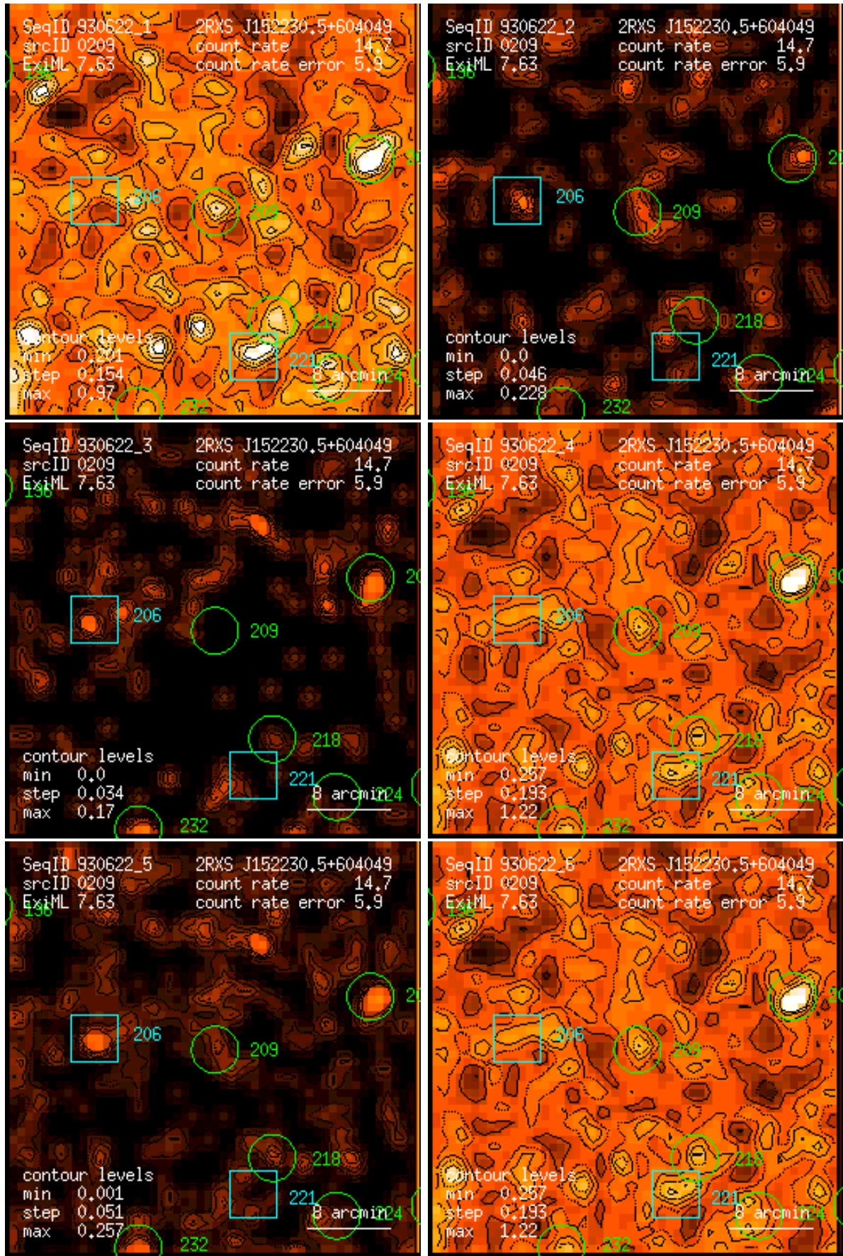
Figure 209: RASS 930622: detection 0209: band rate images, Gaussian filter: (1) PSPC channels 11 – 41, (2) 52 – 90, (3) 91 – 201, (4) 11 – 235, (5) 52 – 201, (6) 11 – 201. Broad band rates in counts/ks. Band rate contour levels in counts/ks/arcmin 2 .
