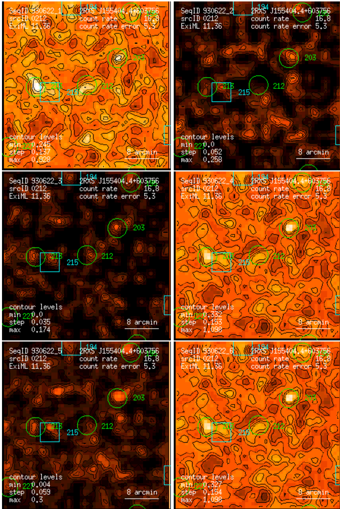
Figure 212: RASS 930622: detection 0212: band rate images, Gaussian filter: (1) PSPC channels 11 – 41, (2) 52 – 90, (3) 91 – 201, (4) 11 – 235, (5) 52 – 201, (6) 11 – 201. Broad band rates in counts/ks. Band rate contour levels in counts/ks/arcmin 2 .
