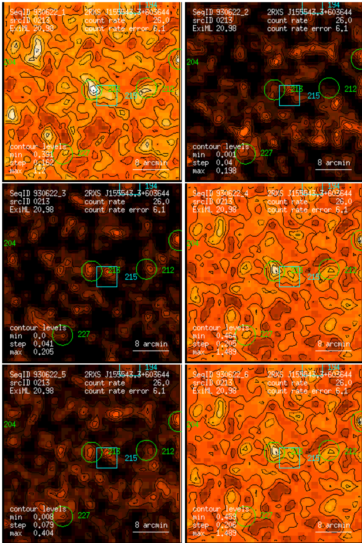
Figure 213: RASS 930622: detection 0213: band rate images, Gaussian filter: (1) PSPC channels 11 – 41, (2) 52 – 90, (3) 91 – 201, (4) 11 – 235, (5) 52 – 201, (6) 11 – 201. Broad band rates in counts/ks. Band rate contour levels in counts/ks/arcmin 2 .
